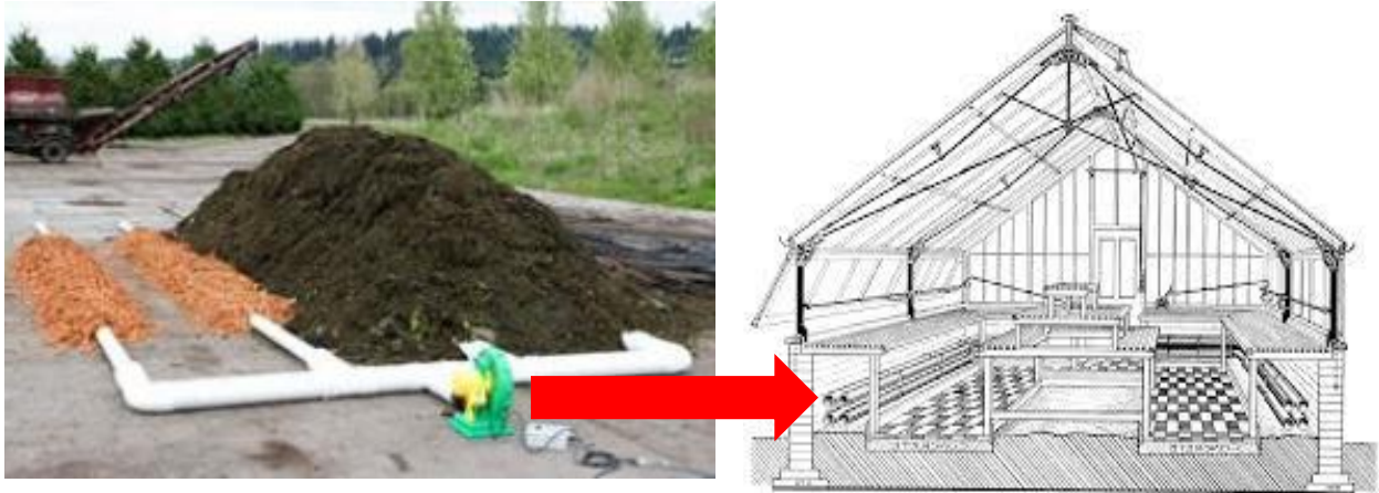
Figure E.3. Conceptual diagram of a high tunnel/greenhouse system heated by direct piping of vapor from an ASP system into heat transfer pipes within the structure.
