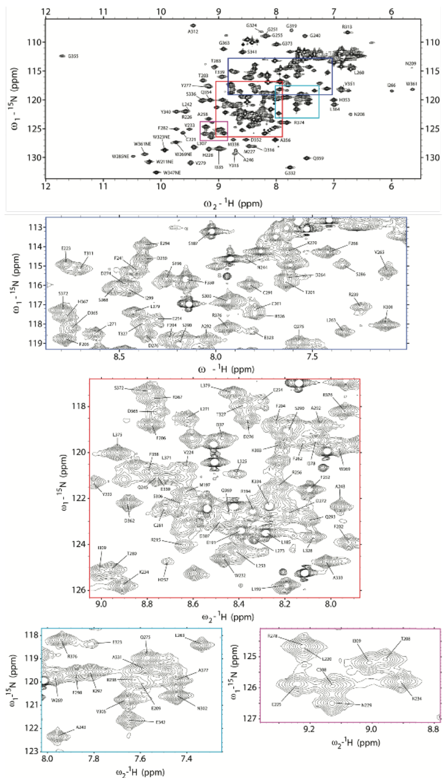
Figure 5.1: NMR signal assignments of A3Gctd-2K3A-E259A at pH 6.0. ^1\text{H} - ^{15}\text{N} HSQC spectrum of A3Gctd-2K3A-E259A. Inset locations indicated with colored boxes correspond to expanded inset spectrum borders.
