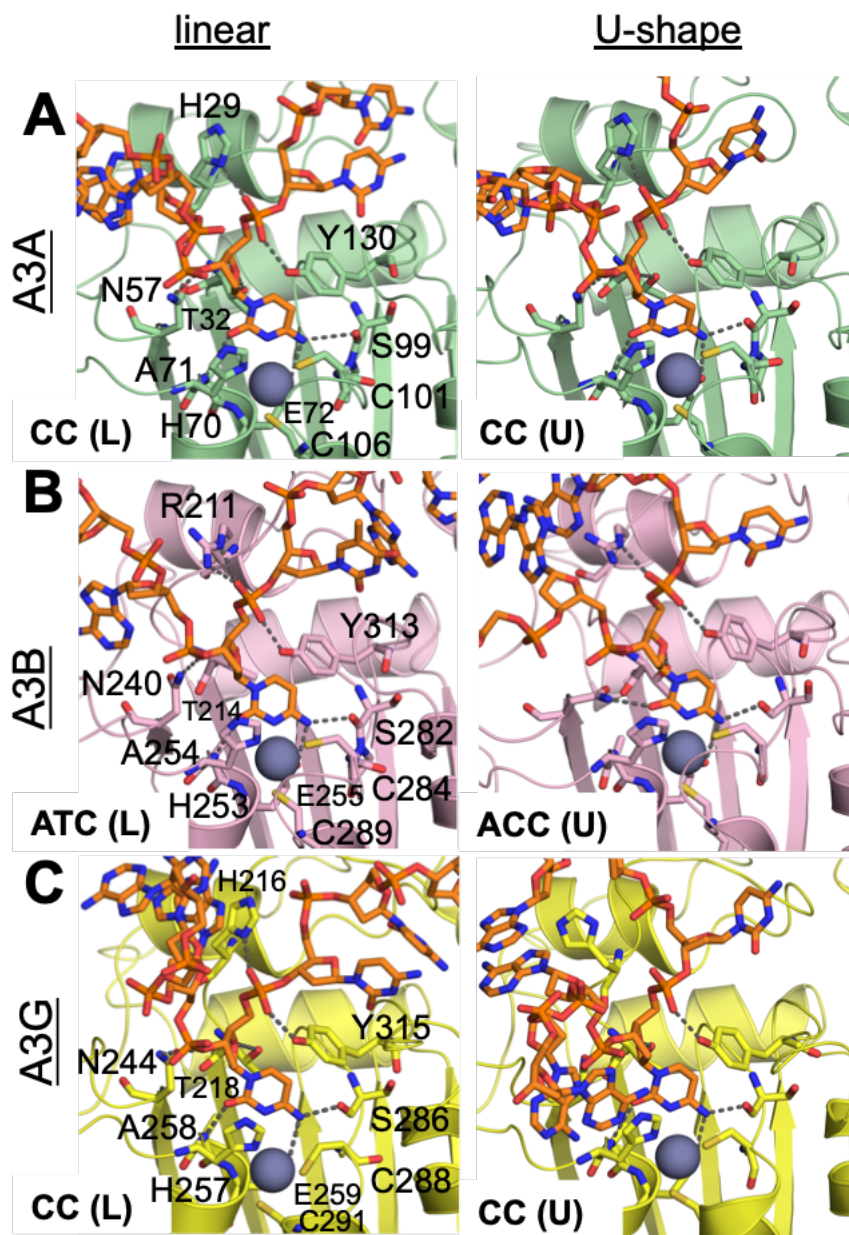
Figure 3.3: The interactions between target cytidine and active site residues in MD simulations of linear and U-shaped ssDNA.
