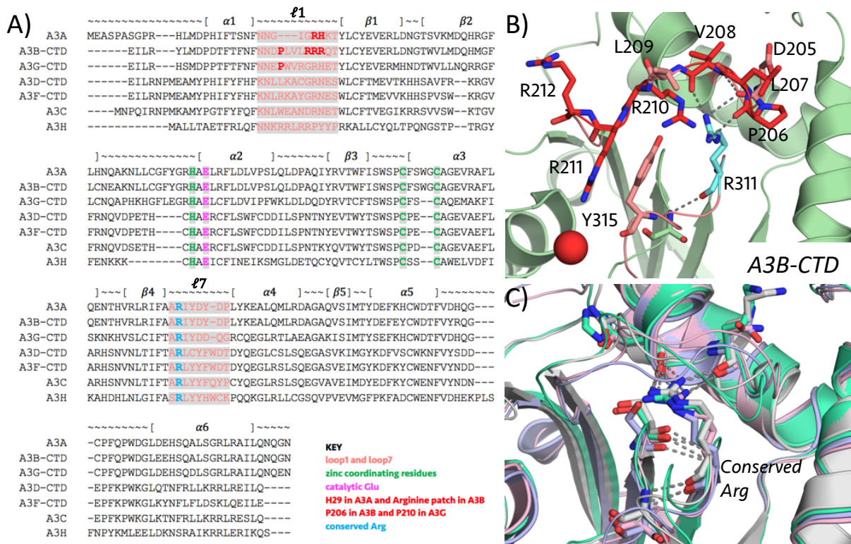
Figure 2.8: Amino acid sequence and structural differences between A3B-CTD and catalytically active A3 domains.
