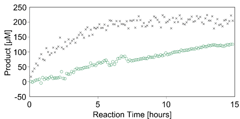
Figure 5.8: Deamination of rC and dC by A3A.
