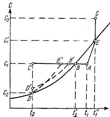
Figure 1.1 - Solubility diagram
