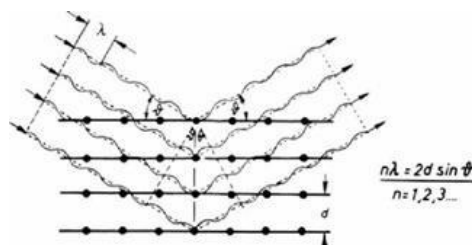
Figure 1.3 - The Wulf-Bragg diffraction condition.
