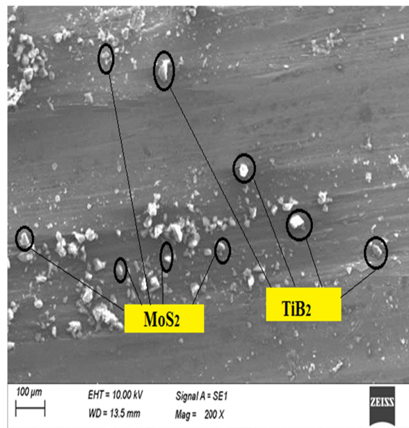
Fig. 5.c Al7075-12%TiB 2 -1.5MoS 2
