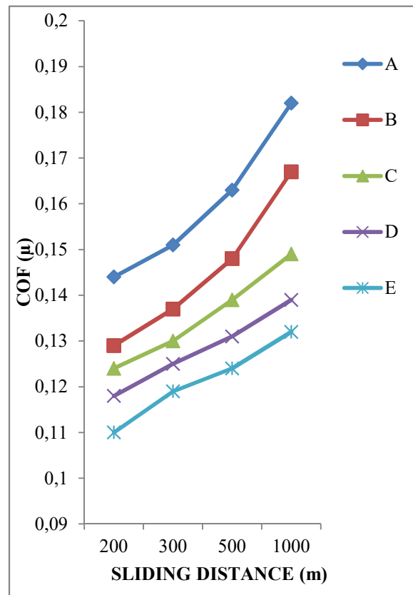
Fig. 7.f Sliding distance vs COF
