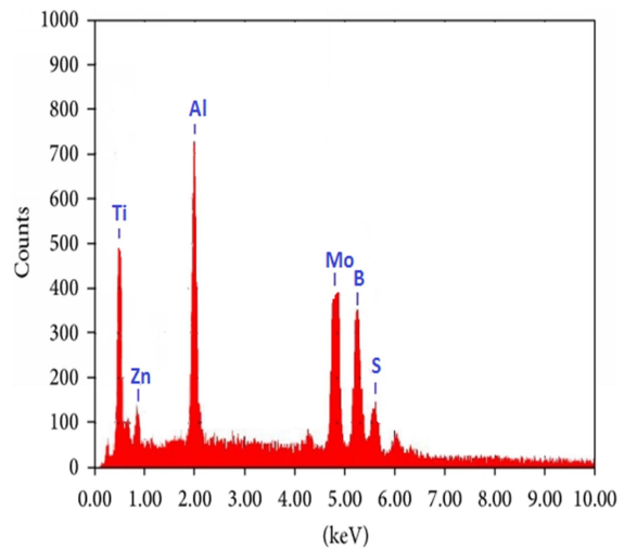
Fig. 4.e AL7075-12%TiB 2 -4.5%MoS 2
