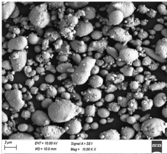
Fig. 1 Al7075 powders
