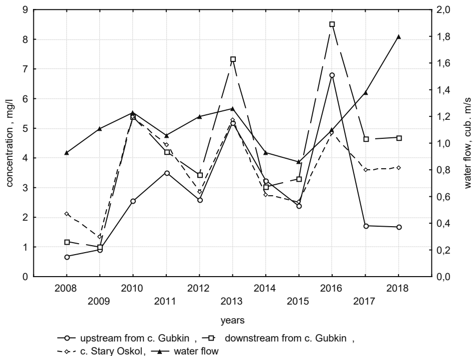
Fig. 1. Nitrate content in Oskolets river (Roshydromet) for 2008–2018
