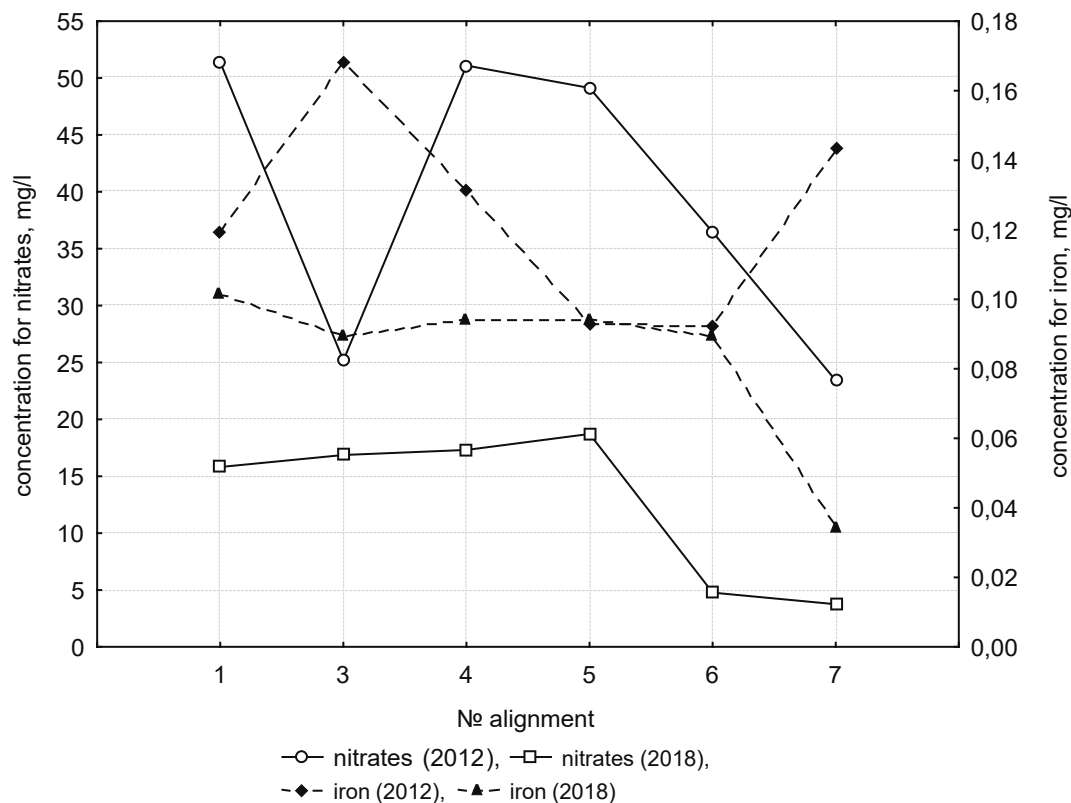
Fig. 5. The pollutants content per sections in Oskolets river for 2012–2018 (database fragment)
