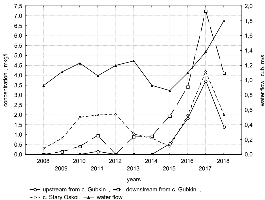
Fig. 2. Zinc content in Oskolets river (Roshydromet) for 2008–2018
