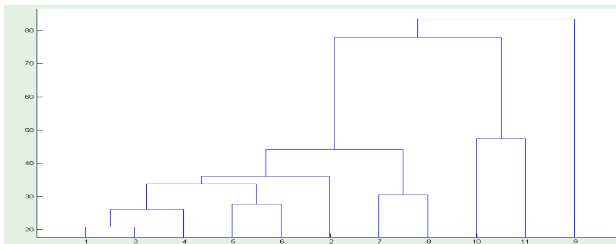
Fig. 3. Grouping of average annual hydroecological situations on Oskolets river of the Belgorod Region (from 1 to 11 years of observations for the corresponding period from 2008 to 2018)
