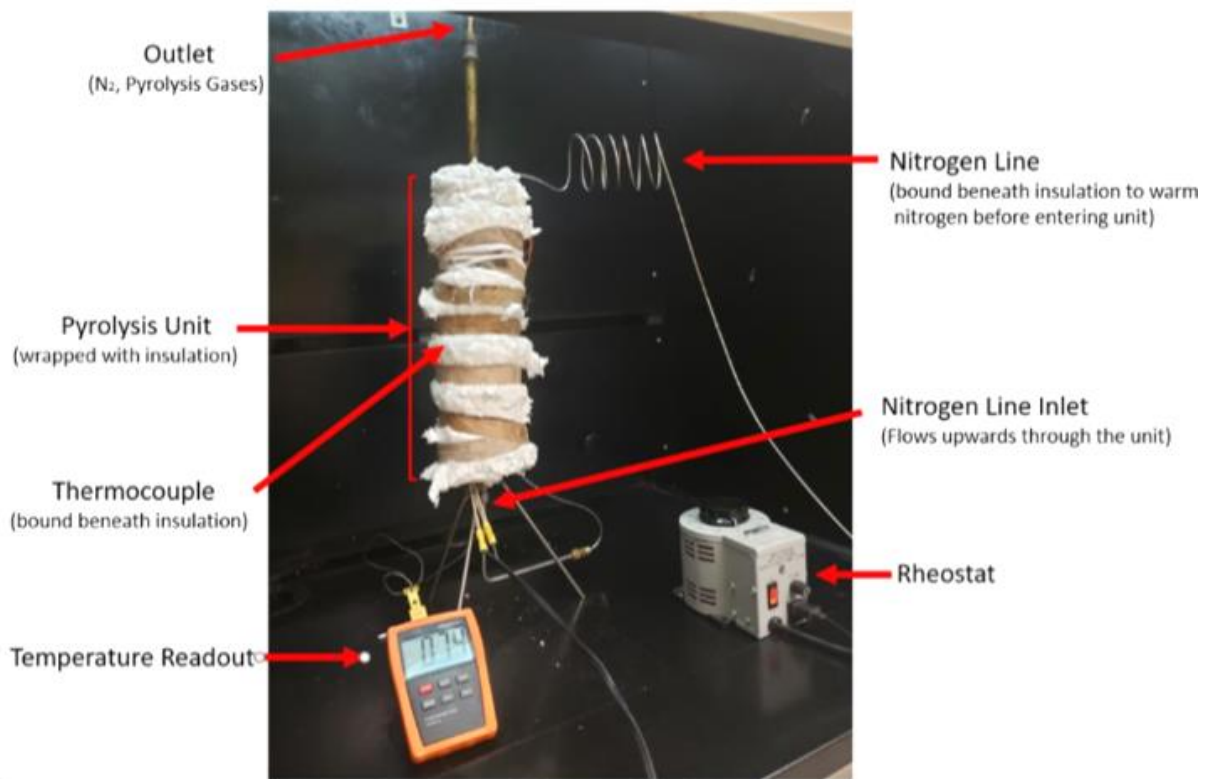
Figure 2: Pyrolysis Unit
