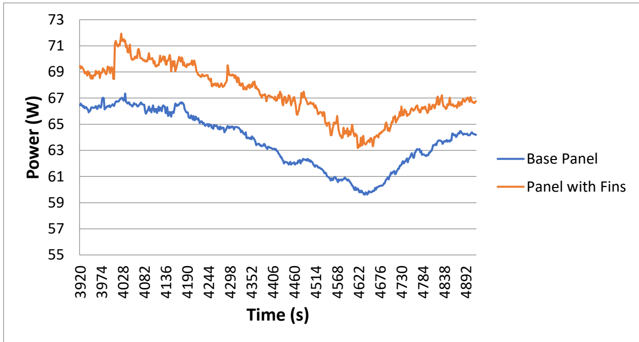
Figure 23. Power vs Time graph for a base panel and the panel with fins during the same experiment shown in Figure 22.
