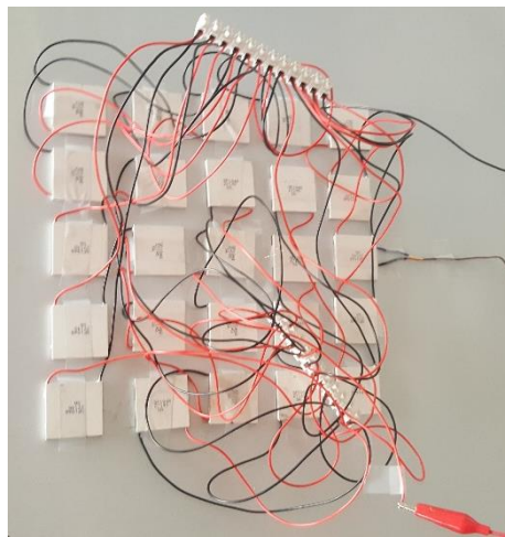
Figures 16. TEG setup with fins
