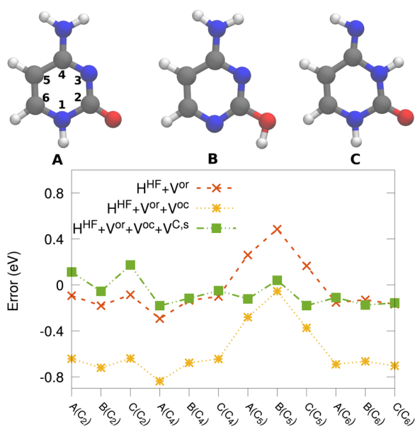
FIG. 17. (Top) Tautomers of cytosine considered in this study. The following color scheme was used for the atoms: H (white), C (gray), N (blue), and O (red). (Bottom) Errors in d -GKS-srRPA based C(1s) CEBEs for cytosine tautomers compared to CVS-ADC(4) values. 264 HF exchange is denoted as HF. For the d -GKS-srRPA calculations, def2-TZVPP basis sets and the PBE potential (grid size m5) were used. The molecular geometries were optimized using the PBE energy functional. Reprinted with permission from Voora et al. , J. Chem. Phys. 151 , 134106 (2019). Copyright 2019 AIP Publishing LLC.
