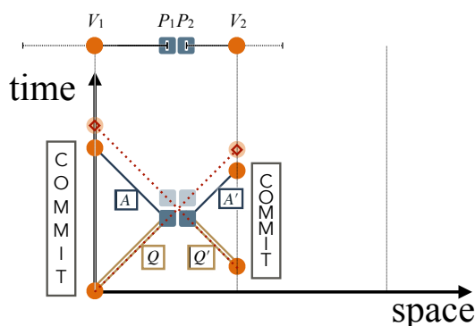
■ Figure 2 Space-Time diagram of our ZK-MIP* for NP. ( 45^\circ diagonals are the speed of light.)
