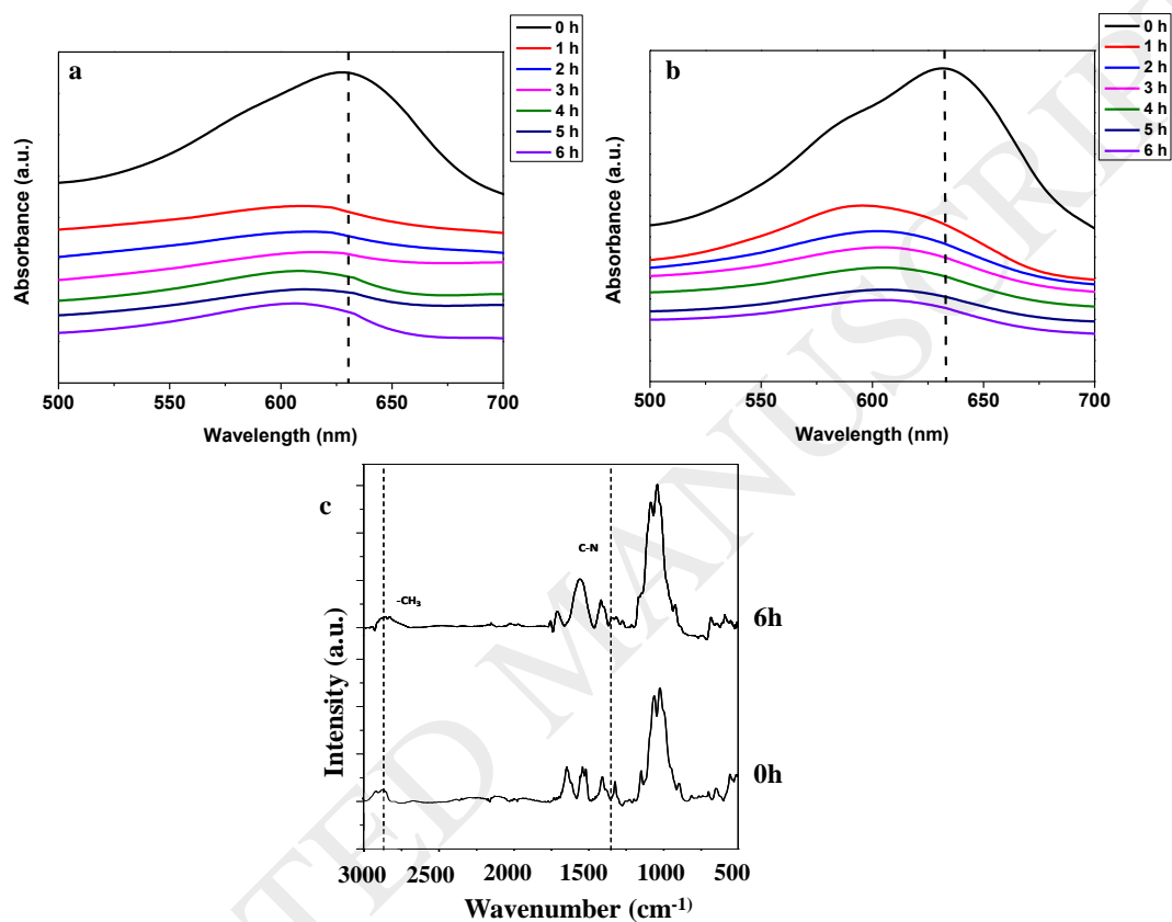
Figure 10. Evolution of malachite green main light band absorption at 624 nm during UV-A+Visible light irradiation in (a) 70QS/30UTiO 2 -10 film. (b) 50QS/50UTiO 2 -10 film. (c) Attenuated total reflection Malachite green IR peaks monitored by Fourier transform infrared spectroscopy (ATR-FTIR) spectrum in 70QS/30UTiO 2 -10 film. Subtraction of chitosan and UTiO 2 IR bands were achieved.
