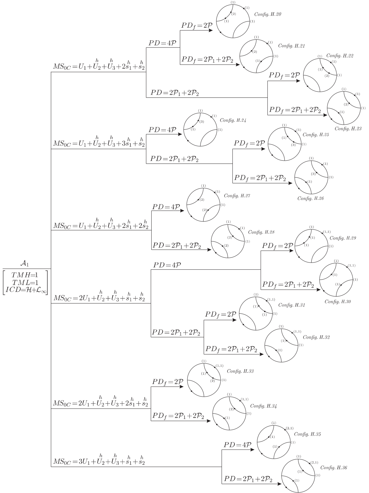
DIAGRAM 3: (Cont.) Diagram of configurations with one hyperbola and TMH = 1
