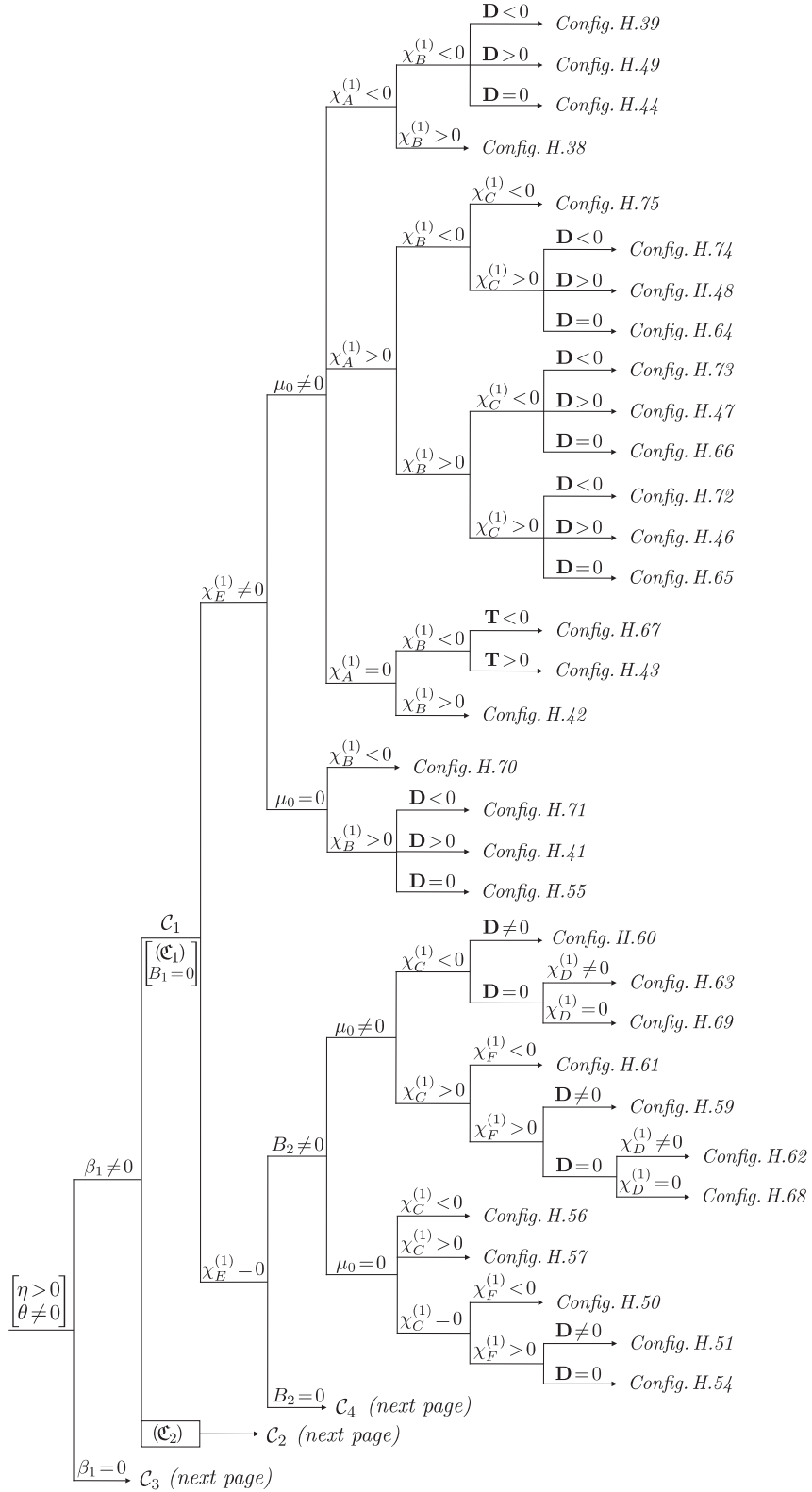
DIAGRAM 10: (Cont.) Bifurcation diagram in \mathbb{R}^{12} of the configurations: Case \eta > 0 , \theta \neq 0
