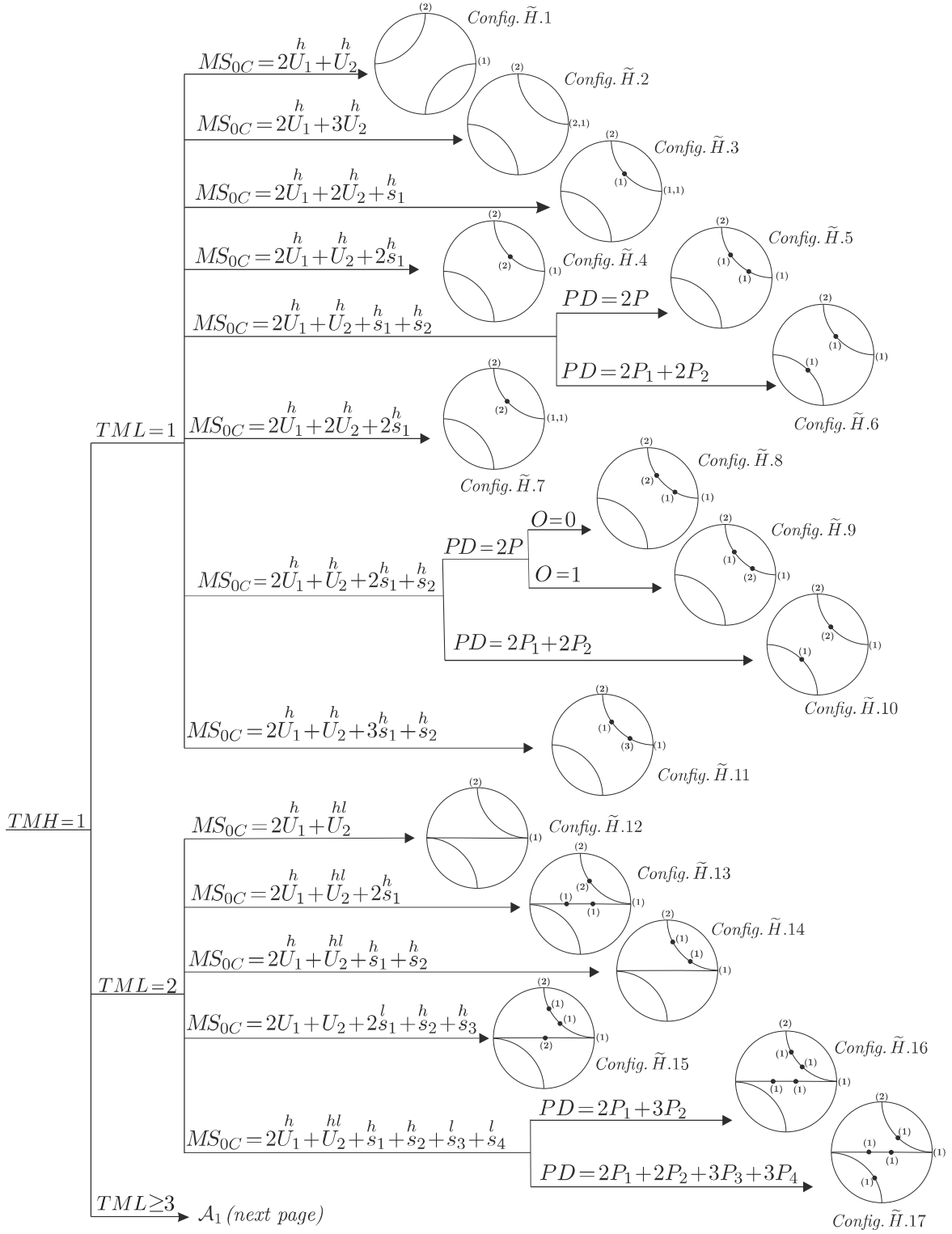
DIAGRAM 12: Diagram of configurations with one simple hyperbola
