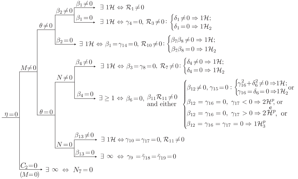
DIAGRAM 2: Existence of invariant hyperboloids: the case \eta = 0
