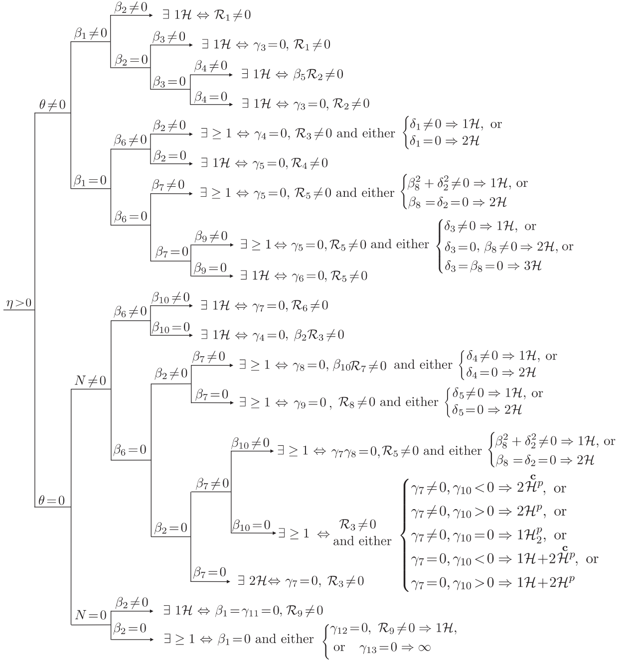
DIAGRAM 1: Existence of invariant hyperboloids: the case \eta > 0
