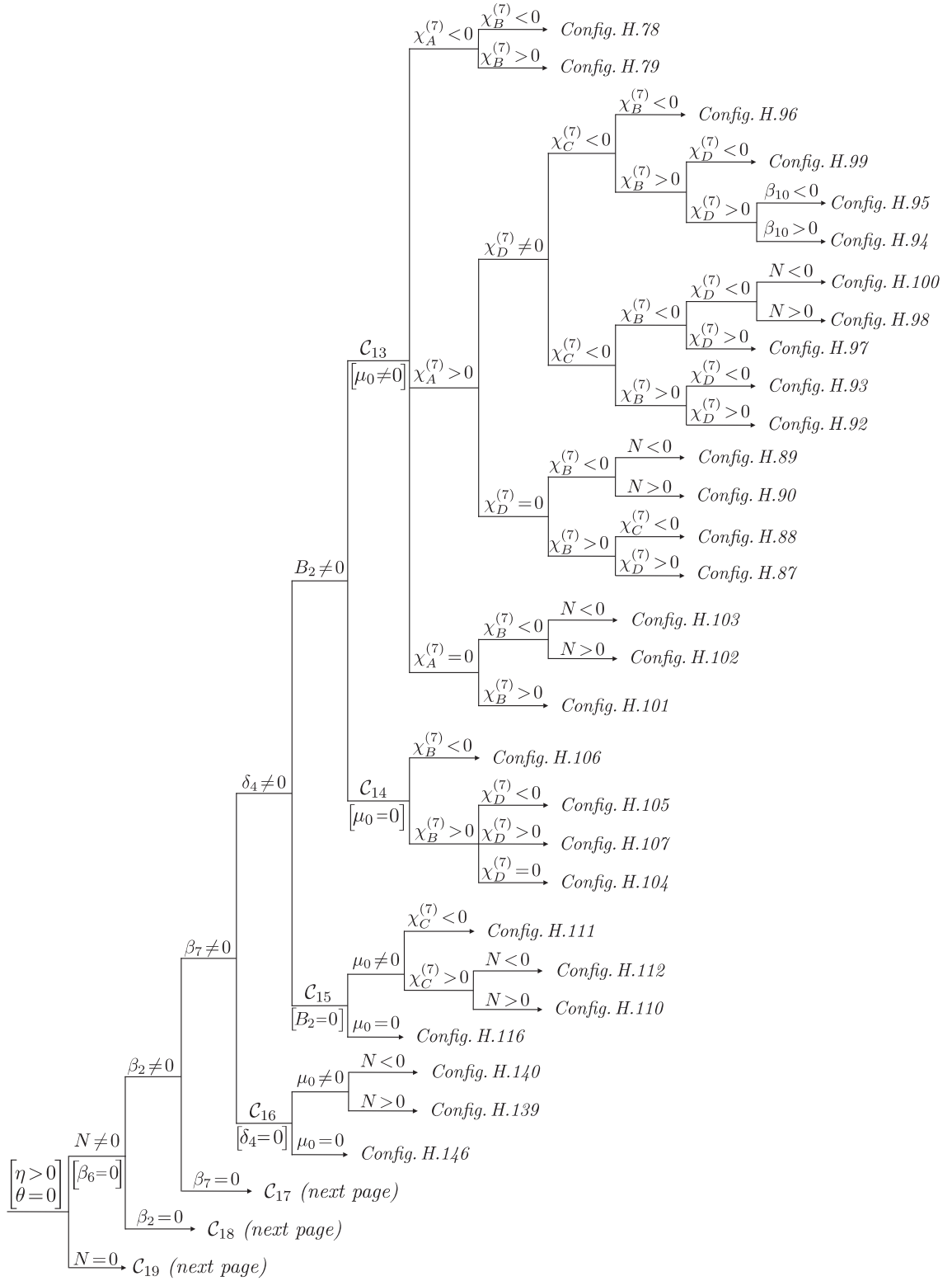
DIAGRAM 11: (Cont.) Bifurcation diagram in \mathbb{R}^{12} of the configurations: Case \eta > 0 , \theta = 0
