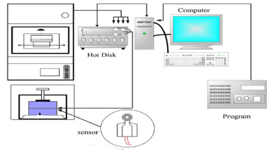
Fig 1 - Basic layout of the apparatus, (Al-Ajlan, 2006).
