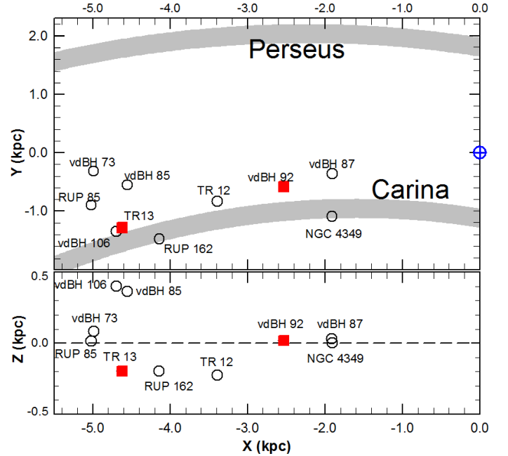
Fig. 17. X – Y (upper panel) and X – Z (lower plane) projection of the true and probable clusters in our sample (open circles). The red squares enclose the youngest clusters in our list (see Table 4). The thick gray lines in the upper panel show the trace of the Perseus and Carina arms according to Vallée (2005). The position of the Sun is shown by a blue crossed circle. The dashed line in the lower panel depicts the Galactic equator.
