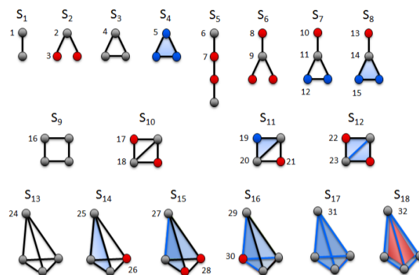
Fig. 2. Illustration of 2- to 4-nodes simplices. The 18 2- to 4-nodes simplices are denoted by S_1 to S_{18} . Within each simplex, geometrically interchangeable nodes, belonging to the same orbit, have the same color. These simplices have 32 different orbits, denoted from 1 to 32. Note that simplices S_4 , S_8 , S_{11} and S_{14} have only one 2D face (triangle, in blue), while S_{12} and S_{15} have two triangles, S_{16} has 3 triangles and S_{17} has four triangles. S_{18} has four triangles and one 3D face (tetrahedron, in red).
