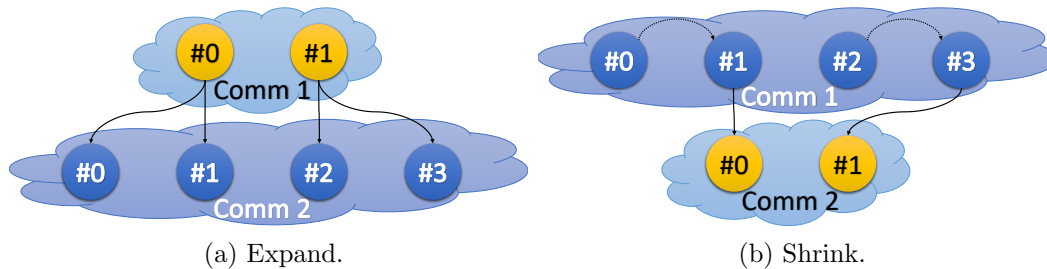
Figure 2: Data transfers.
