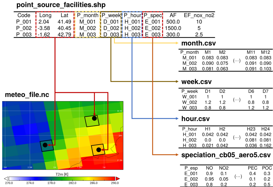
Figure 2. Illustration of how the different input files used by the point source sector are linked and cross-referenced. The multipoint shapefile ( point_source_facilities.shp ), contains temporal and speciation profile IDs for each facility (e.g. “MXXX” for the monthly profiles, “XXX” being a three-digit numeric code that starts at “001”), which are cross-referenced with the corresponding temporal and speciation CSV files ( month.csv , week.csv , hour.csv , speciation_cb05_aero5.csv ). The shapefile also contains the geographical coordinates of each facility (long, lat), which are used to identify the closest grid cell of the meteorological NetCDF file ( meteo_file.nc ) and derive the surface temperature data.
