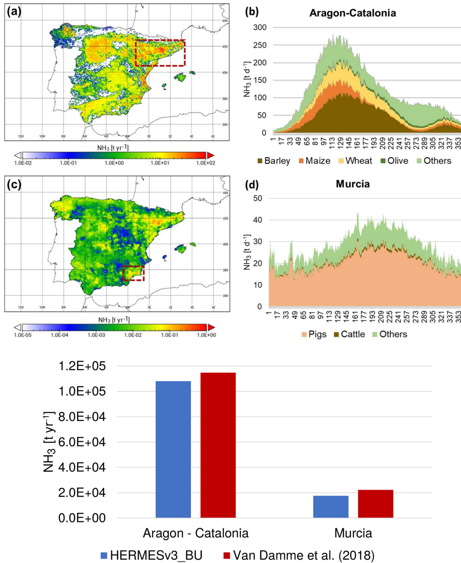
Figure 6. Spanish annual \text{NH}_3 (a) fertilizer and (c) livestock emissions ( \text{t yr}^{-1} ) calculated on a Lambert conformal conic grid of 4 km by 4 km resolution and corresponding time series of daily \text{NH}_3 ( \text{t d}^{-1} ) for the regions of (b) Aragon and Catalonia per crop type and (d) Murcia per livestock category; (e) the total \text{NH}_3 emissions (fertilizers+livestock) estimated for these two hot spots ( \text{t yr}^{-1} ) are compared against IASI satellite-derived \text{NH}_3 emission fluxes (Van Damme et al., 2018).
