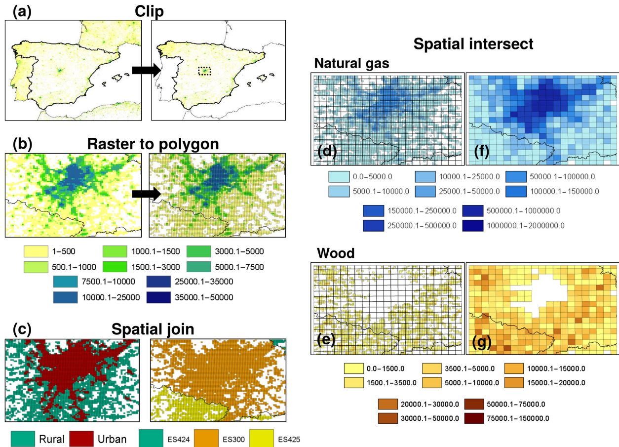
Figure 3. Examples of the spatial operations performed by HERMESv3_BU during the initialization of the residential and commercial combustion emission sector, including (a) a clip of the original GHSL population density raster (population per pixel) using a shapefile of the administrative borders of Spain, (b) a conversion of the clipped raster to a polygon feature (population per cell) (zoom over the area of Madrid), (c) the spatial joins performed to append the NUTS3 administrative boundary codes (ES300, Madrid; ES424, Guadalajara and ES425, Toledo) and the GHSL settlement categories (urban, rural) to each source grid cell, and the spatial intersections applied to remap the fuel consumption data (natural gas in urban and rural areas and wood in rural areas) (GJ per cell per year) from the source (d, f) domain to the user-defined (e, g) destination domain (4 km by 4 km Lambert conformal conic grid).
