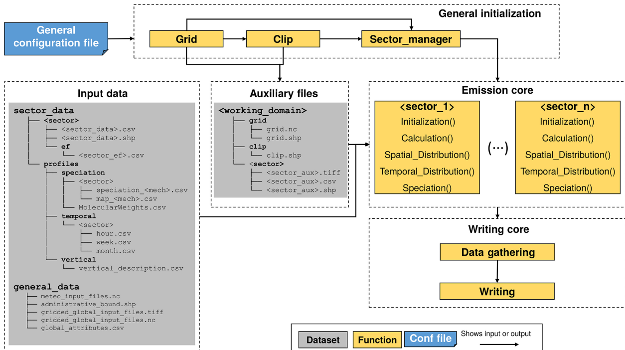
Figure 1. Schematic representation of the general structure of HERMESv3_BU. All the parameters described by the user in the general configuration file (e.g. working domain, execution dates, input data paths) are used to execute the initialization process (i.e. creation of working grid, clip polygon and auxiliary files and distribution of the computational resources). Once the general initialization is finished, HERMESv3_BU starts the execution of the emission core of the model. For each pollutant sector, and considering the input data provided by the user, HERMESv3_BU performs a (i) sector initialization, (ii) sector calculation, (iii) spatial mapping, (iv) temporal distribution and (v) speciation. Once the emission estimation of all sectors is finished, the writing core proceeds to gather all the data and writing it according to the atmospheric chemistry output format selected by the user.
