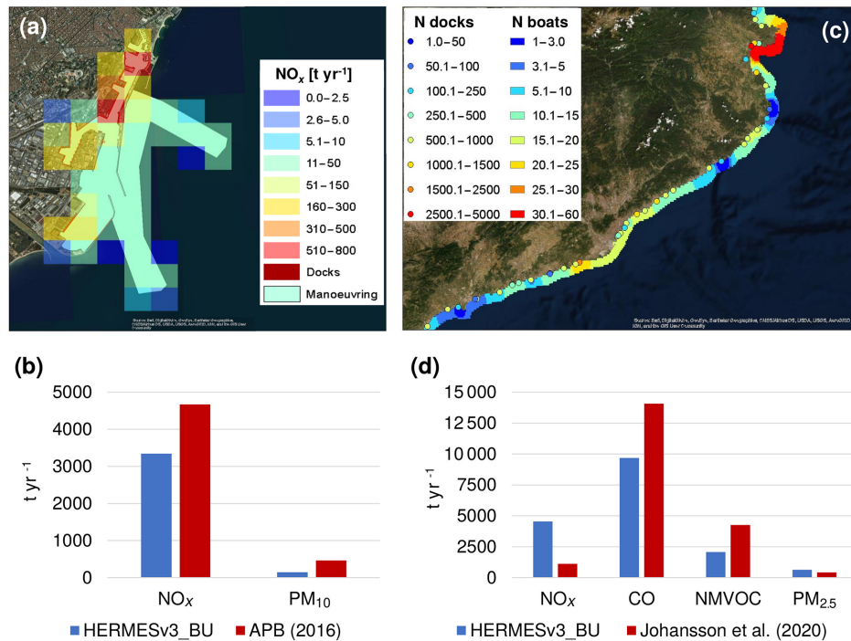
Figure 7. (a) Annual \text{NO}_x emissions ( \text{t yr}^{-1} ) for the Port of Barcelona calculated on a regular 1 km by 1 km grid. Dark red and light blue layers represent the spatial proxies used to allocate hotelling and manoeuvring emissions, respectively. (b) Comparison between annual \text{NO}_x and \text{PM}_{10} of Barcelona's port emissions ( \text{t yr}^{-1} ) estimated with HERMESv3_BU and reported by the Barcelona Port Authority inventory (APB, 2016). (c) Spatial distribution of Spanish marinas (with the associated number of docks) and recreational boats along the Costa Brava region (coast of Catalonia). (d) Comparison between annual \text{NO}_x , CO, NMVOC and \text{PM}_{2.5} pleasure boat emissions ( \text{t yr}^{-1} ) estimated for Spain (HERMESv3_BU) and the Baltic Sea region (Johansson et al., 2020). (Sources of the ArcGIS Online basemap: Esri, DigitalGlobe, GeoEye, i-cubed, USDA FSA, USGS, AEX, Getmapping, Aerogrid, IGN, IGP, swisstopo and the GIS user community. Maps in (a) and (b) were created using ArcGIS® software by Esri. ArcGIS® and ArcMap™ are the intellectual property of Esri and are used herein under license. Copyright © Esri. All rights reserved. For more information about Esri® software, please visit https://www.esri.com (last access: February 2020).)
