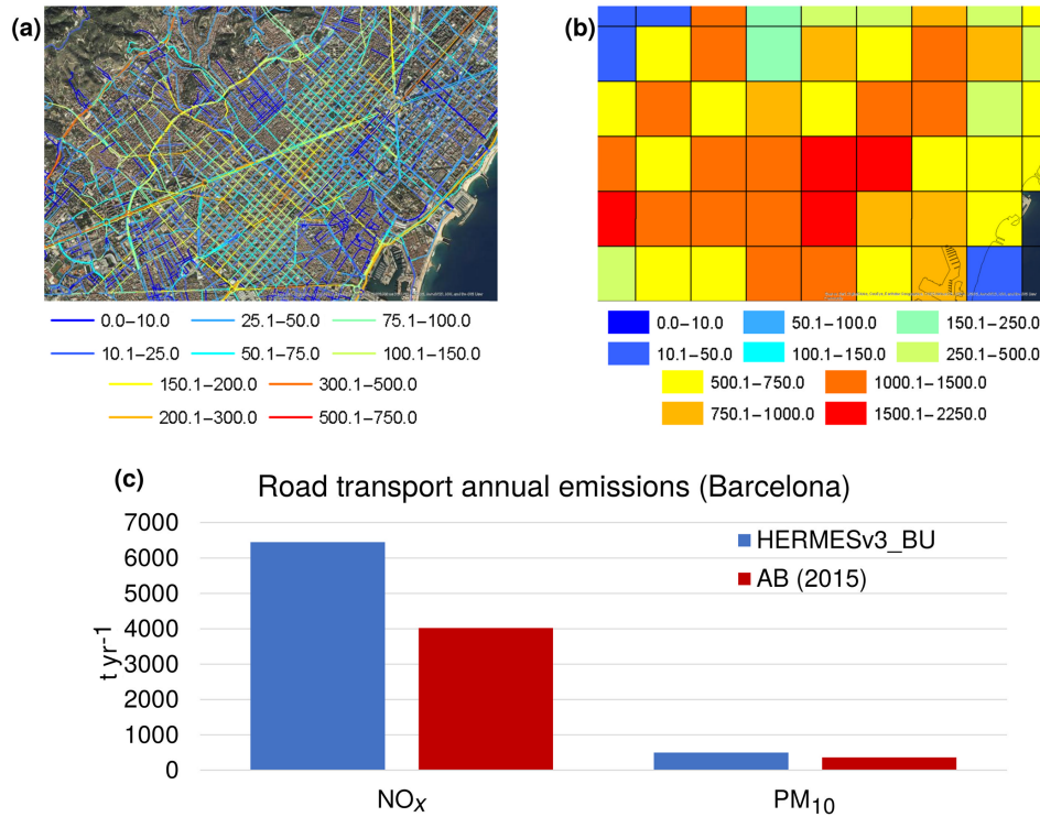
Figure 5. Hourly PM 2.5 road transport emissions estimated for an area of Barcelona city (09:00 UTC) at (a) the road link level (kg km -1 h -1 ) and (b) grid cell level (1 km × 1 km) (kg h -1 ) (sources of the ArcGIS Online basemap: Esri, DigitalGlobe, GeoEye, i-cubed, USDA FSA, USGS, AEX, Getmapping, Aerogrid, IGN, IGP, swisstopo and the GIS user community). (c) Barcelona city total annual NO x and PM 10 road transport emissions (t yr -1 ) estimated by HERMESv3_BU and reported by the Barcelona City Council (AB, 2015). Maps in (a) and (b) were created using ArcGIS ® software by Esri. ArcGIS ® and ArcMap ™ are the intellectual property of Esri and are used herein under license. Copyright © Esri. All rights reserved. For more information about Esri ® software, please visit https://www.esri.com (last access: February 2020).
