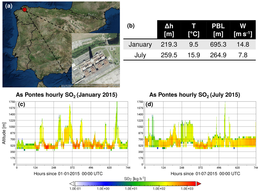
Figure 4. (a) Location of the As Pontes Spanish coal-fired power plant (sources of the ArcGIS Online basemap: Esri, DigitalGlobe, GeoEye, i-cubed, USDA FSA, USGS, AEX, Getmapping, Aerogrid, IGN, IGP, swisstopo and the GIS user community); (b) modelled average plume thickness ( \Delta h ) (m), air temperature at the stack height ( T ) (°C), boundary-layer height (planetary boundary layer, PBL) (m) and wind speed at the stack height ( W ) (m s -1 ) for January and July (monthly averages); results of the hourly and vertically distributed SO 2 emissions (kg h -1 ) estimated by HERMESv3_BU for the months of (c) January and (d) July 2015. The map in (a) was created using ArcGIS ® software by Esri. ArcGIS ® and ArcMap ™ are the intellectual property of Esri and are used herein under license. Copyright © Esri. All rights reserved. For more information about Esri ® software, please visit https://www.esri.com (last access: February 2020).
