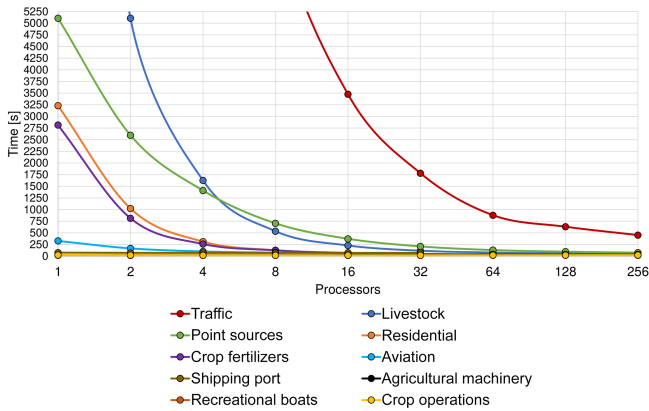
Figure 9. Computational times (s) obtained from the scalability test performed with HERMESv3_BU over Spain. Each line represents the amount of time needed to complete the emission estimation process of each pollutant sector as a function of the number of processors used ( x axis, represented with a base 2 logarithmic scale).
