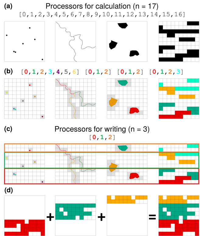
Figure 8. Illustrative example of how HERMESv3_BU parallelizes the calculation and writing processes and distributes the computational resources. (a) A total of 17 processors are selected to estimate emissions from point sources, road transport, aviation and an area source sector (e.g. residential combustion). (b) The calculation processors are distributed as follows: seven for the point sources (one processor per facility), three for road transport (one processor per road link), three for aviation (one processor per polygon) and four for residential combustion (one processor per subgroup of cells equally balanced, i.e. 10 cells per subgroup). Each processor estimates the emissions of the corresponding partitioned element and maps them onto the intersected grid cells (highlighted in grey). (c) During the writing process, HERMESv3_BU decompose the destination working domain into three horizontal sections (equivalent to the number of writing processors selected), maintaining each row as indivisible. (d) For each horizontal section, the model gathers the estimated gridded emissions of all the sources involved in that section and then computes the total sum per grid cell. Once this operation is finished, the resulting emissions are dumped into the corresponding section of the output file.
