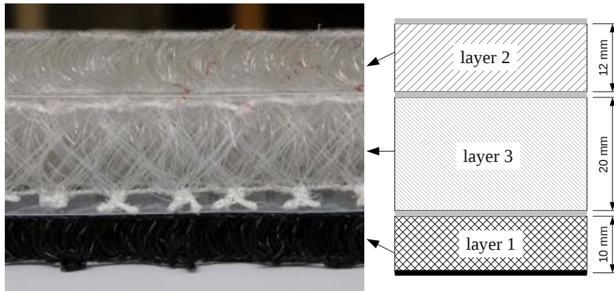
Figure 2: Thermal collector composed of 3 layers of textile spacer fabrics.
