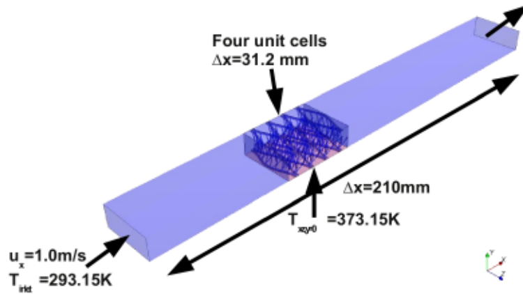
Figure 8: Geometry and boundary conditions (LC2).
