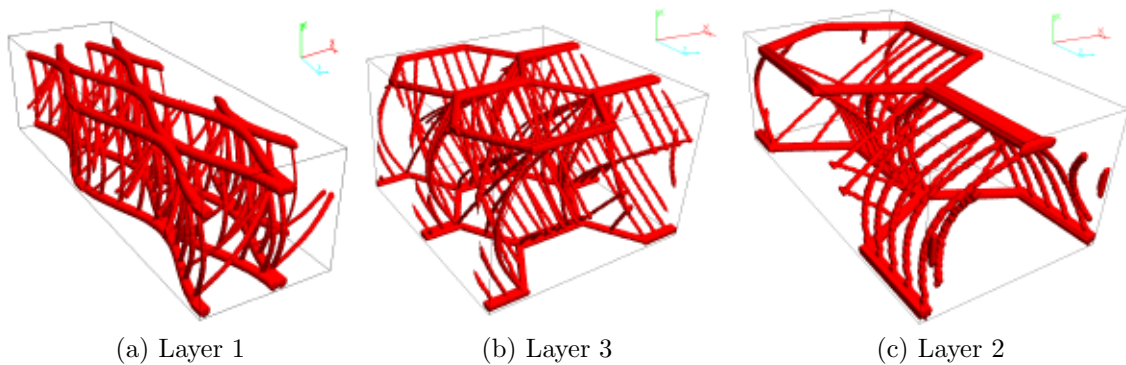
Figure 5: Modeled layers of the thermal collector.
