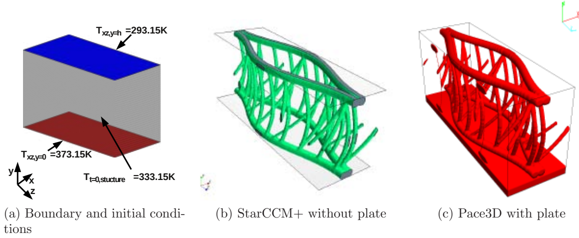
Figure 7: Boundary conditions and simulation environment (LC1).
