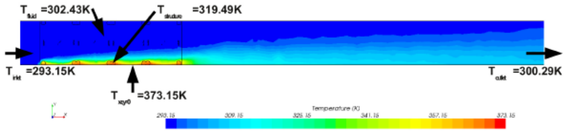
Figure 10: Temperature distribution in the xy -layer (LC2).
