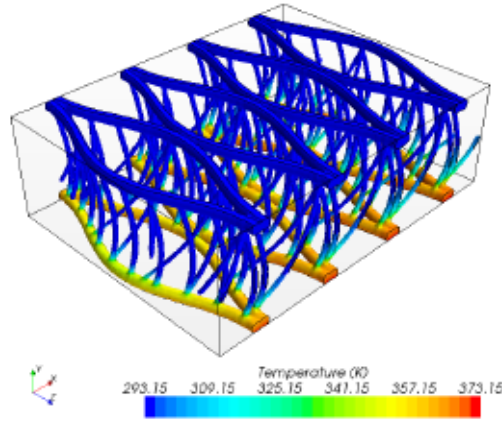
Figure 12: Temperature distribution in the textile fiber.
