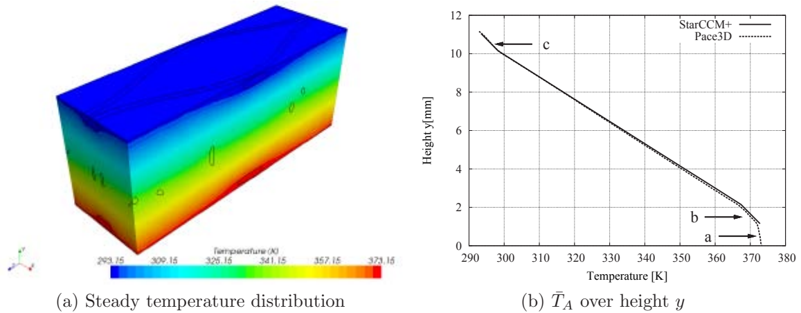
Figure 9: Temperature distribution and profile.
