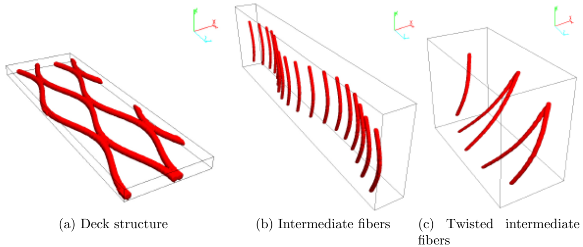
Figure 4: Design elements to construct layer 1.
