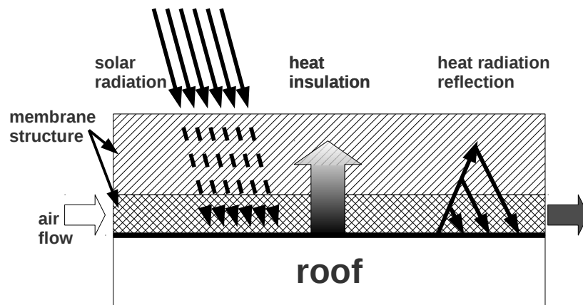
Figure 1: Design and principle of a thermal collector with membrane structures.
