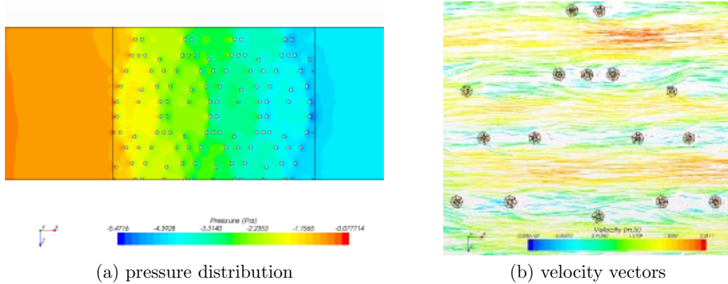
Figure 11: Pressure distribution and velocity vectors for the xz -layer (LC2).
