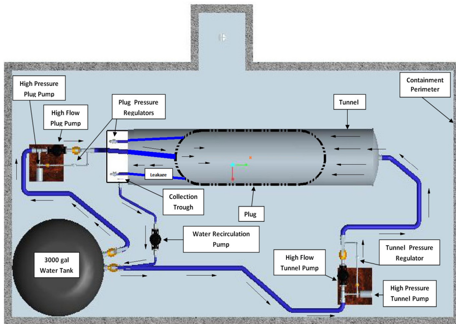
Figure 2: Plan view of the reduced-scale flooding simulation system used for testing.
