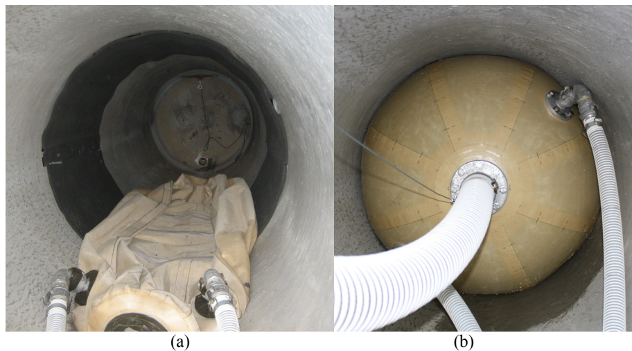
Figure 4: (a) Example of neoprene tunnel lining positioned in the cylindrical portion of the deflated plug; (b) Inflated plug positioned for testing.
