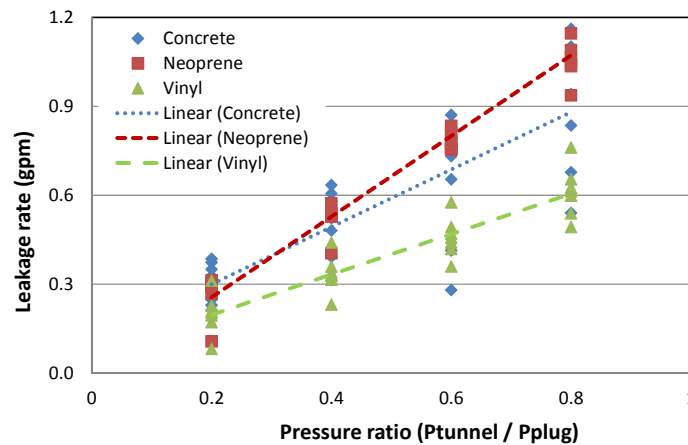
Figure 8: Leakage rate vs. Pressure ratio.
