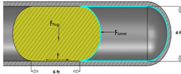
Figure 6: Forces acting on the testing system.
