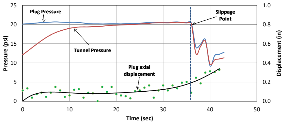
Figure 5: Example of plug and tunnel pressures variation as well as axial displacement up to the point of slippage.
