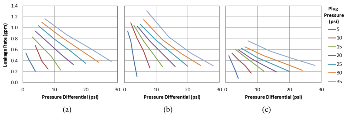
Figure 7: Leakage rate for: (a) Concrete; (b) Neoprene; (c) Vinyl.
