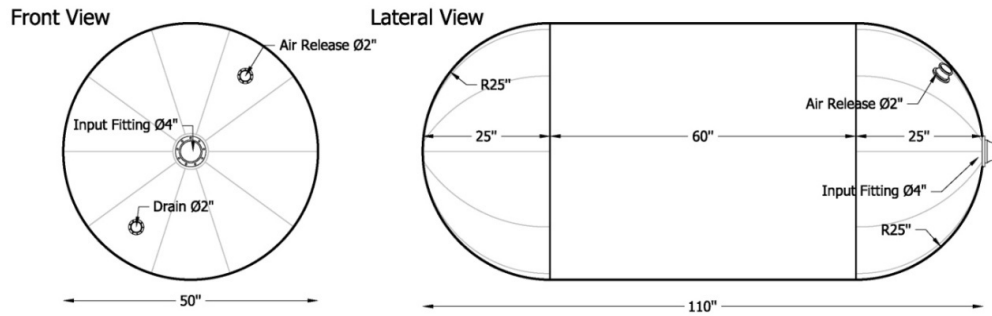
Figure 1: Inflatable plug general dimensions (1 inch = 2.54 cm).
