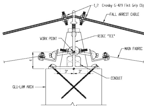
Figure 6: Blackwell top of arch detail (section & isometric)
