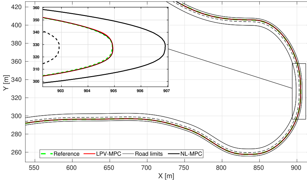
Figure 3. Simulation circuit used for testing the proposed control technique (LPV-MPC) and its non-linear version (NL-MPC).
