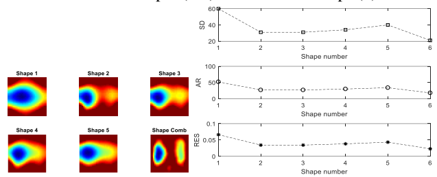
Fig. 7. Reconstruction of two inclusions one large for case (c), one small, bottom rows reconstruction of shapes 1-5 from Fig. 2, and (6) is when the shapes are combined. Top right shows the image quality measures from five shapes (1-5) and combined shape (6)
