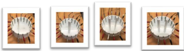
Fig.4 Four experimental set up, case a small inclusion in left, a large inclusion in centre/left, one large and one small inclusions centre/right, and two large inclusions right
