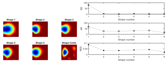
Fig. 5. Reconstruction of single inclusion at top left for case (a), bottom rows reconstruction of shapes 1-5 from Fig. 2, same inclusion in all 5 shapes in the same position, and (6) is when the shapes are combined. Top right shows the image quality measures from five shapes (1-5) and combined shape (6)
