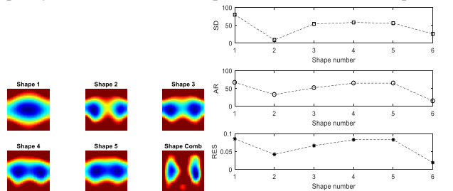
Fig. 8. Reconstruction of two equal size inclusions for case (d), bottom rows reconstruction of shapes 1-5 from Fig. 2, and (6) is when the shapes are all combined. Top right shows the image quality measures from five shapes (1-5) and combined shape (6)
