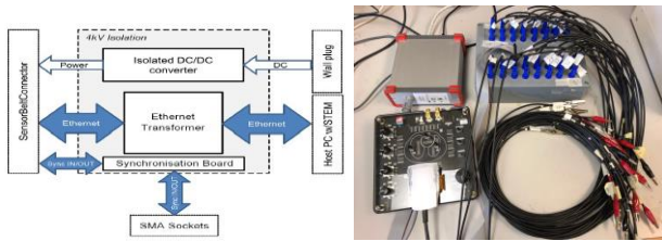
Fig. 3: The block diagram of data collection module and sensor
