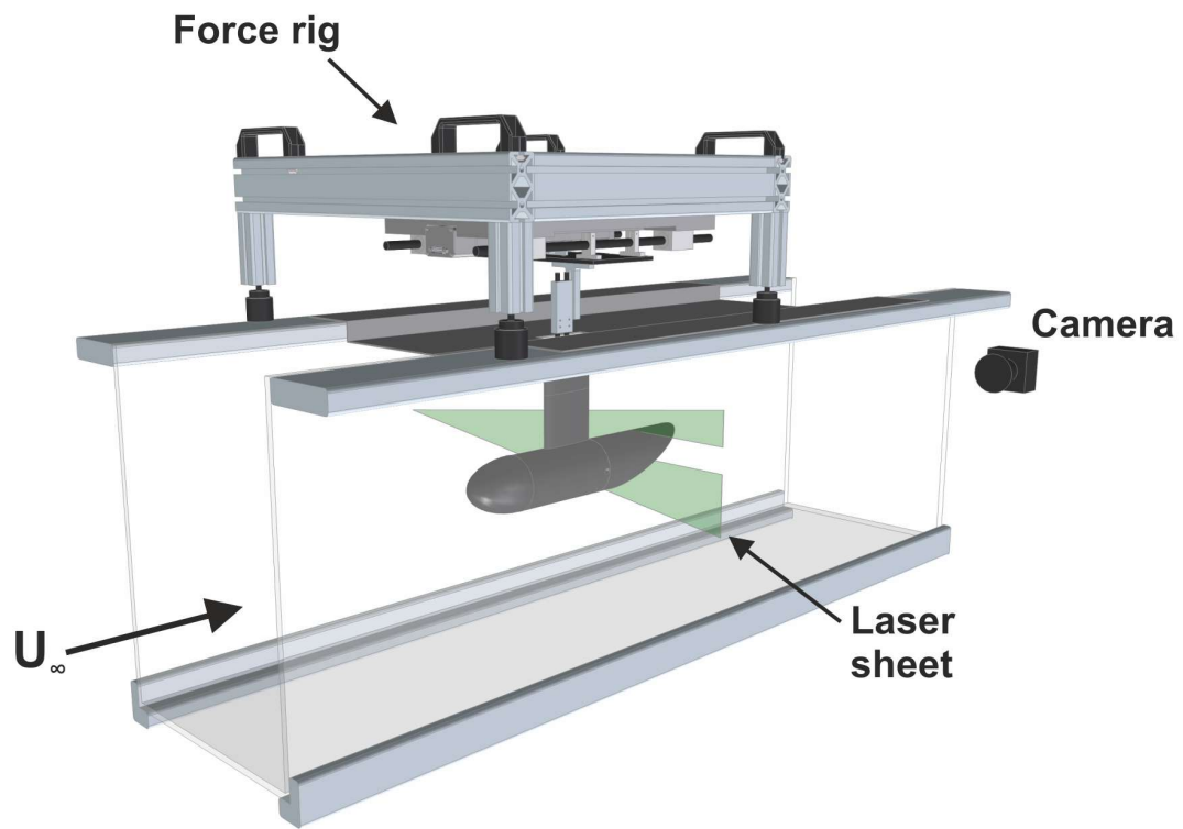
Figure 1. A schematic of the experimental setup in the water tunnel, showing the laser and camera positions for crossflow PIV measurements.
