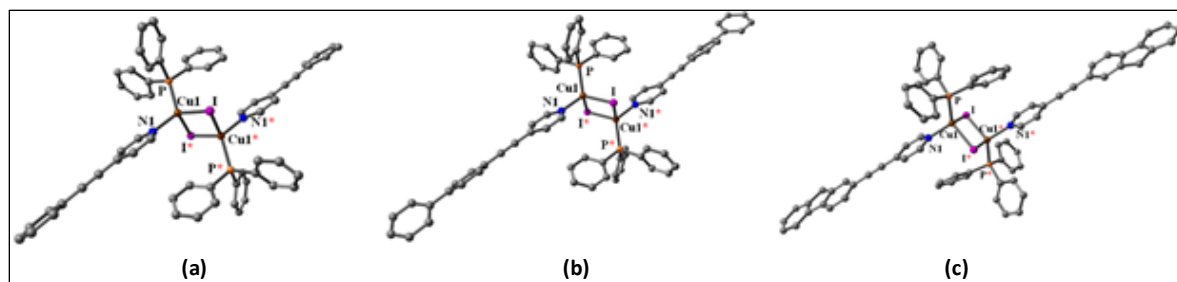
Figure 4. DFT optimized structures of (a) C_1 , (b) C_2 , and (c) C_3 .
