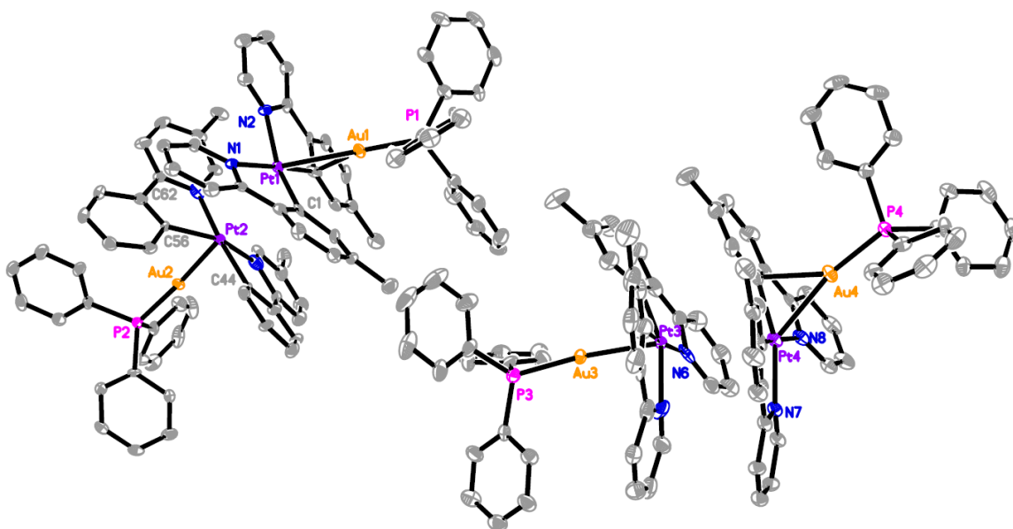
Figure 4. Molecular structure of complex 4 . The triflate anions, solvents of crystallization and H atoms were omitted for clarity.
