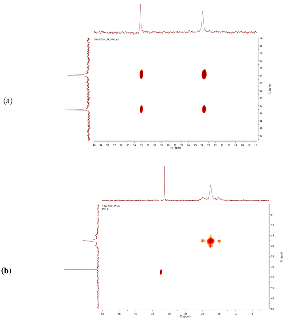
Figure 6. The ^{31}\text{P}\{^1\text{H}\} EXSY NMR spectrum of 4 in acetone- d_6 at (a) 213 and (b) 193 K.
