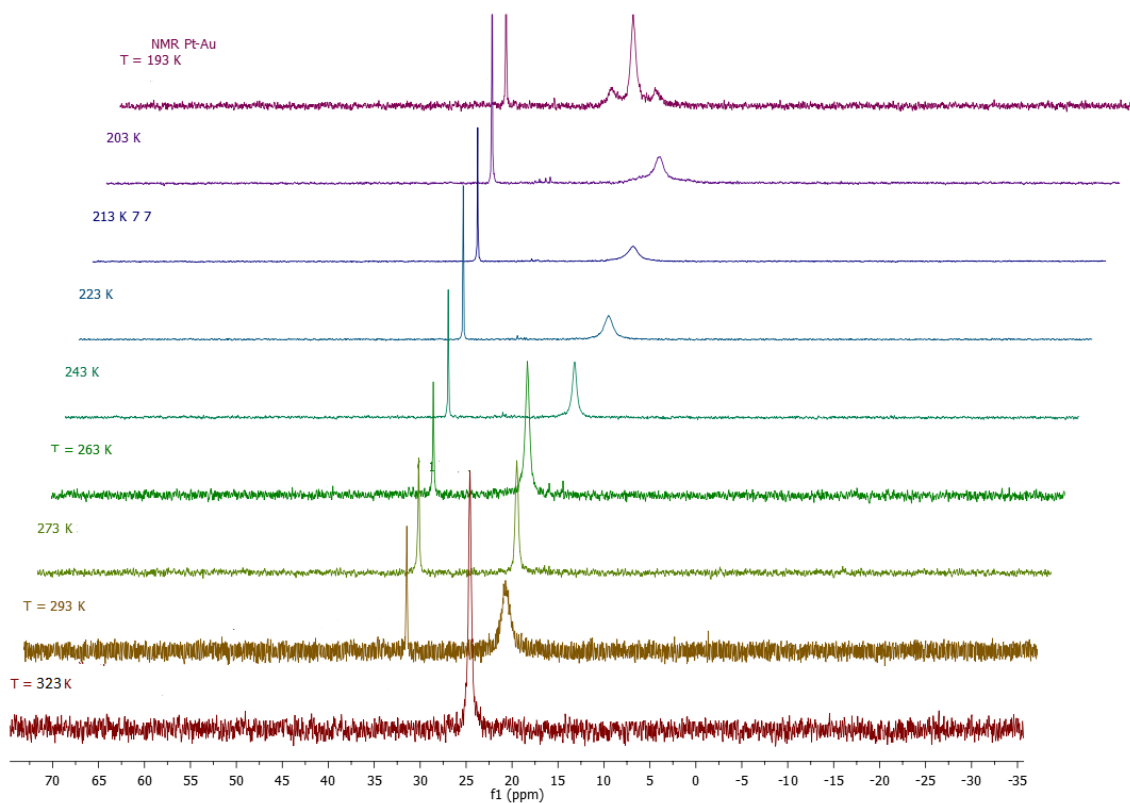
Figure 5. VT ^{31}\text{P}\{^1\text{H}\} NMR spectrum of complex 4 in acetone- \text{d}_6
