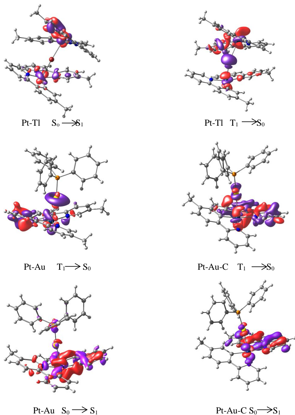
Figure 9. PBE0-DFT transition densities for the lowest-energy singlet excitations and triplet emissions of 3 and 4 . During the electronic transition, the electron density increases in the blue areas and decreases in the red areas.
