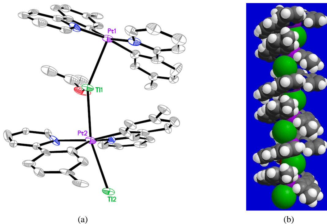
Figure 2. A view of asymmetric unit of 3 (a) and its helical chain structure along a axis (b). The anions (PF 6 ), solvents of crystallization and H atoms are omitted for clarity.
