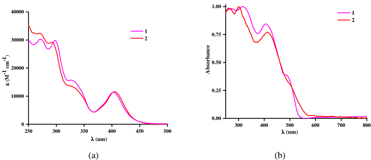
Figure 7. (a) Absorption spectra in \text{CH}_2\text{Cl}_2 (concentration = 5 \times 10^{-5} M) (b) Diffuse reflectance UV-vis spectra in the solid state of complexes 1 and 2 at 298 K
