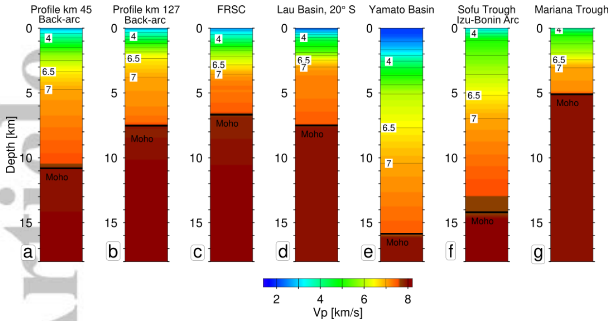
Figure 11. Comparison of 1D velocity profiles from the back-arc and FRSC with profiles from other back-arc regions. Profiles a – c from this study and represent averages over a range of 7 km along the profile at indicated locations. d) Represents average back-arc crust near the Eastern Lau Spreading Centre between 20°-21° from Arai and Dunn (2014). e) Represents crust from the Yamato Basin where continental crust is rifted T Sato et al. (2014). f) Represents crust in the Sofu Trough behind the Izu-Bonin Arc, from Takahashi et al. (2011). g) Represents crust in the Mariana Trough behind the Mariana Arc, from Takahashi et al. (2008).
