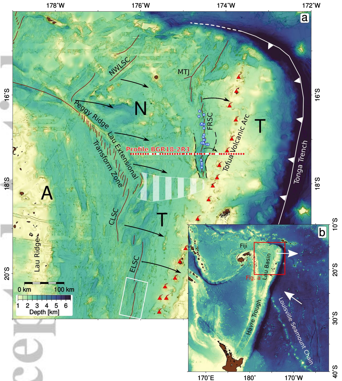
Figure 1. Bathymetry of the northern Lau Basin with tectonic plates and plate boundaries indicated. Map a) shows the Niuafou'ou Microplate (N) with surroundings. A = Australian Plate, CLSC=Central Lau Spreading Centre, ELSC=Eastern Lau Spreading Centre, FRSC = Fonualei Rift and Spreading Centre, MTJ = Mangatolu Triple Junction, NWLSC = Northwestern Lau Spreading Centre, T = Tonga Plate. Our survey line (BGR18-2R3) is plotted as white line with red dots indicating ocean bottom seismometer locations. The black arrows indicate relative sense of plate motions in reference to the Australian Plate, adopted
