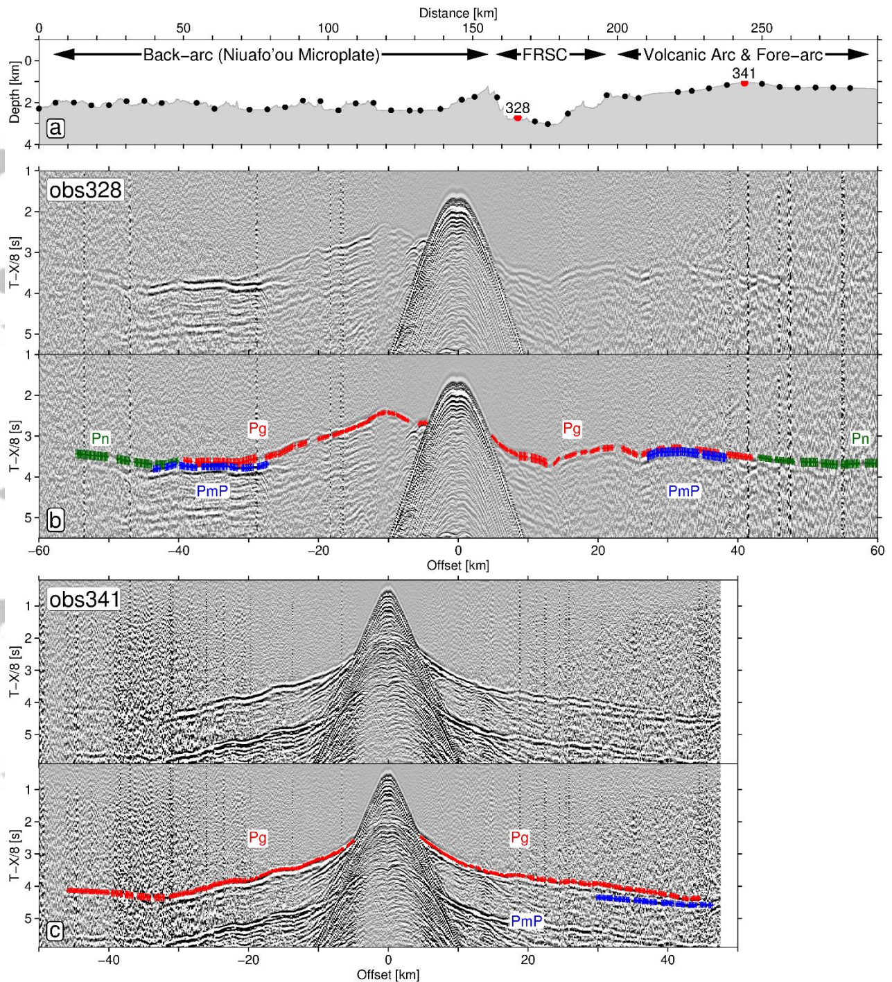
Figure 3. a) Seafloor topography along profile BGR18-2R3 with black dots showing OBS locations. Panels b and c show refraction seismic shot gathers for stations 328 (panel b) within the FRSC and station 341 (panel c) sitting on volcanic-arc crust. Colored bars show phase arrival picks (vertical extent gives uncertainty).
