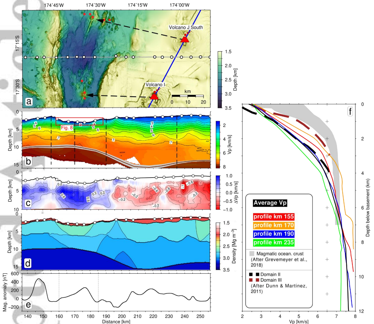
Figure 7. a) Bathymetry of the FRSC and Tonga Arc region with profile BGR18-2R3 (gray line, white circles representing OBS locations). Red trapezoids show locations of arc volcanos and arrows indicate volcanic centers of the FRSC, potentially fed by a common magma reservoir (Sleeper et al., 2016). Solid blue line is the location of the arc volcanic front. Red dots show dredge locations yielding basalts and basaltic andesites (Keller et al., 2008). In terms of geochemistry the dredged lavas are indistinguishable from the lavas of the proximal volcanic arc (Keller et al., 2008). b) Ensemble average P-wave tomography model for the profile section traversing the above map with dashed lines indicating locations of 1D profiles shown in panel f. c) Velocity deviation in the igneous basement from an average 1D Vp-depth profile (solid black line in panel f) in the region between 137-256 km distance. Contours are spaced at 0.2 \text{ km s}^{-1} . Absolute values of calculated Vp deviations deeper than 10
