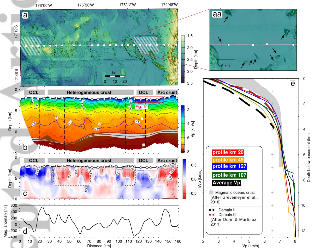
Figure 9. a) Bathymetry of the back-arc region covered by profile BGR18-2R3 (gray line, white circles show OBS locations). Hatched areas indicate regions where the upper crust has a Vp-depth distribution similar to typical oceanic crust. Stippled polygons and lines correspond to polygons in panel c and indicate areas of decreased Vp in the upper crust. It should be noted, that findings from the profile are extrapolated off-profile in the hatched and stippled areas. aa) Zoom-in to the back-arc area covered by sediments. Black arrows indicate locations of small mounds and ridges peeking through the sediment cover which are interpreted to be of volcanic origin. b) P-wave velocity model for the back-arc region with identified sub-domains indicated by gray bars on top. OCL = oceanic crust like. Vertical
