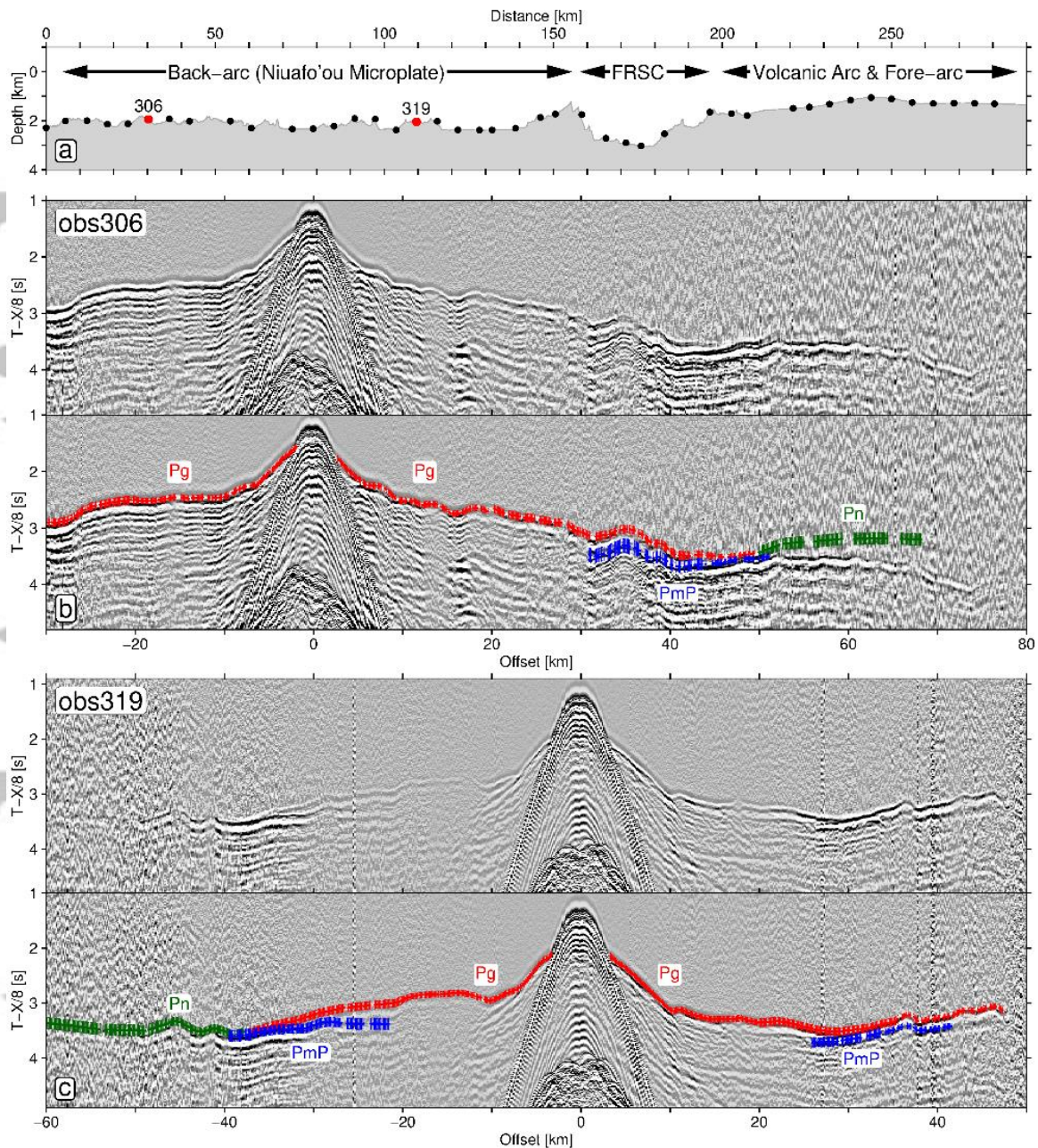
Figure 2. a) Seafloor topography along profile BGR18-2R3 with black dots showing OBS locations. Panels b and c show refraction seismic shot gathers for stations 306 (panel b) and 319 (panel c) sitting on back-arc crust. Colored bars show phase arrival picks (vertical extent gives uncertainty).
