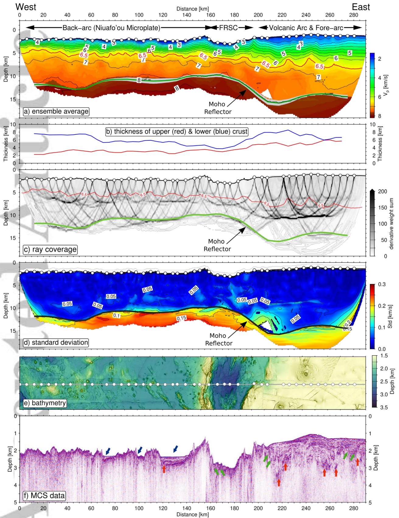
Figure 4. a) Final P-wave tomography model (ensemble average of 100 Monte-Carlo runs) for profile BGR18-2R3 with major tectonic regions indicated on top. Contour interval is 0.5 \text{ km s}^{-1} . We define the 6.5 \text{ km s}^{-1} contour as the boundary between the upper and lower crust
