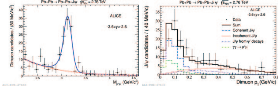
Fig. 1. – Left: invariant mass spectrum of forward ( -3.6 < y < -2.6 ) coherent J/\psi \rightarrow \mu^+\mu^- candidates with p_T < 300 MeV/c and less than 6 neutrons in the ZDC. Right: J/\psi p_T distribution fitted to a simulation template as described in the text. The same distributions for the mid-rapidity region, for the dielectron and dimuon channels are not shown here and can be found in [7].
