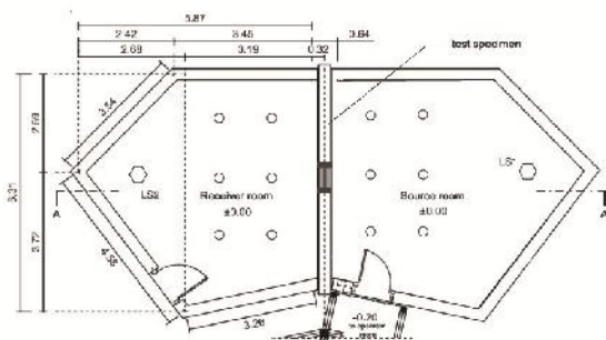
Fig 7. Plan of the testing rooms and the equipment layout.
