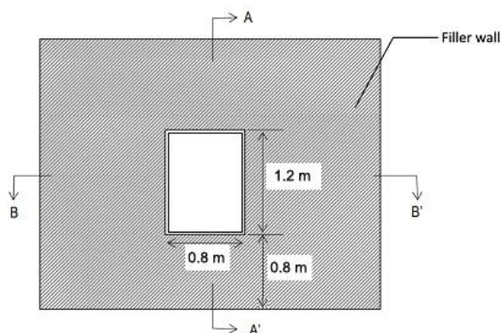
Fig 1. Front view of composite wall specimen.
