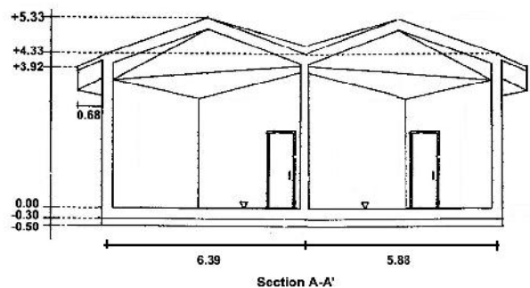
Fig 8. A-A' section of the testing rooms.
