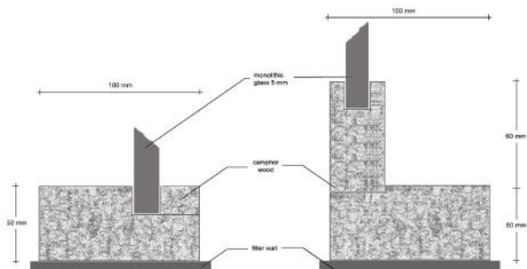
Fig. 4. Detailed section of the timber frame of fixed (left) and open (right).
