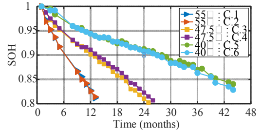
Fig. 5. SOH curves of the tested six cells during the calendar aging at 55°C, 47.5°C, and 40°C.
