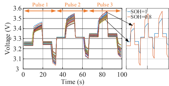
Fig. 6. Voltage datasets obtained during the current pulse tests (as for an example, the aging temperature is 47.5°C).
