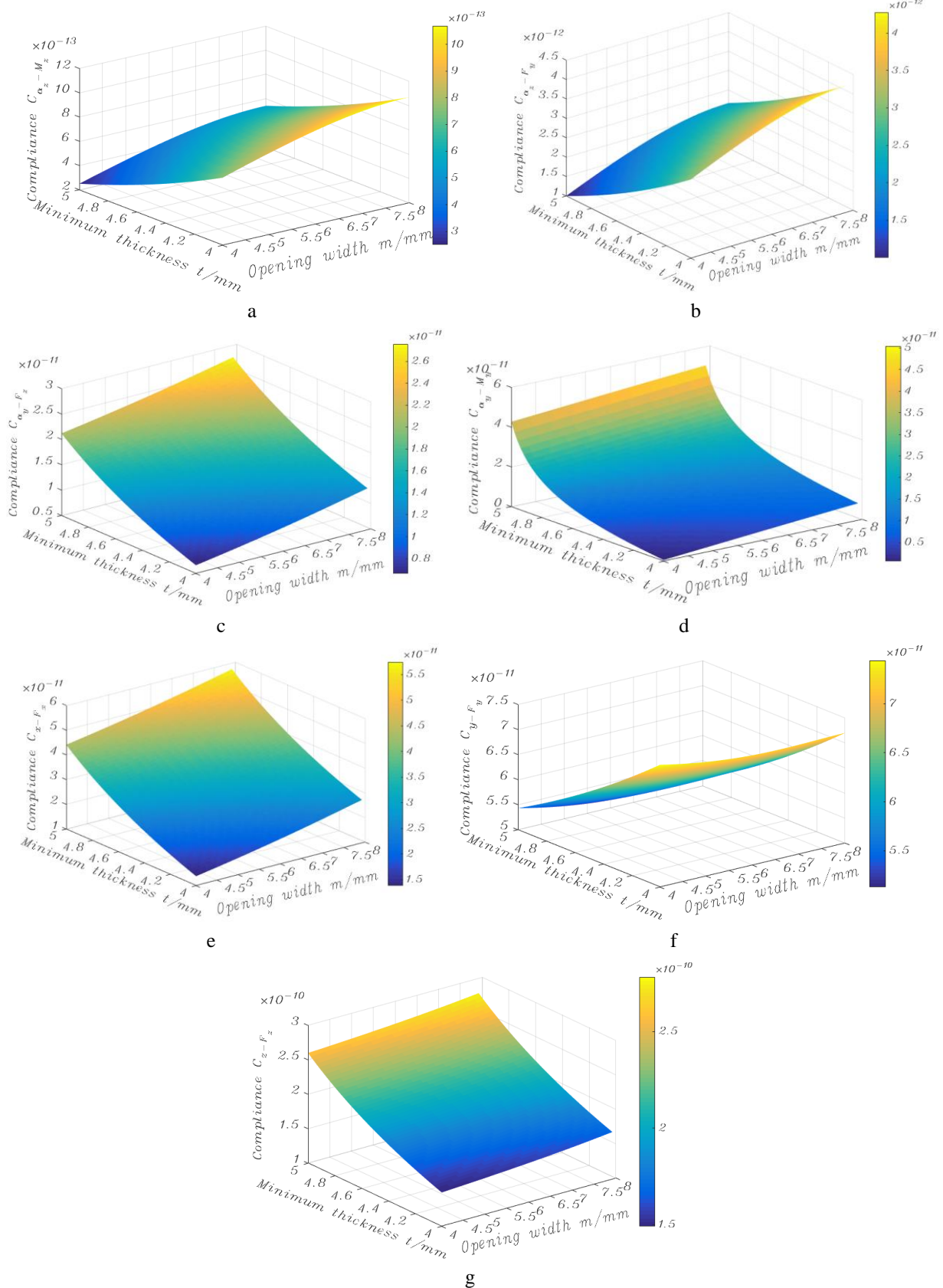
Fig. 6 The influence of parameters m, t on compliance when a \neq b : a – compliance C_{a_z-M_z} ; b – compliance C_{a_z-F_y} ; c – compliance C_{a_y-F_x} ; d – compliance C_{a_y-M_y} ; e – compliance C_{x-F_x} ; f – compliance C_{y-F_y} ; g – compliance C_{z-F_z}
