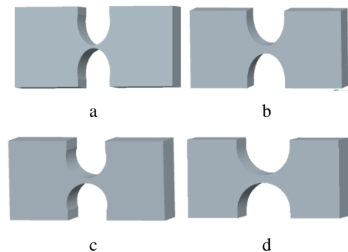
Fig. 1 Four kinds of U-shape flexure hinges with different structures: a – a \neq b and 2b > m ; b – a \neq b and 2b = m ; c – a = b and 2b > m ; d – a = b and 2b = m
