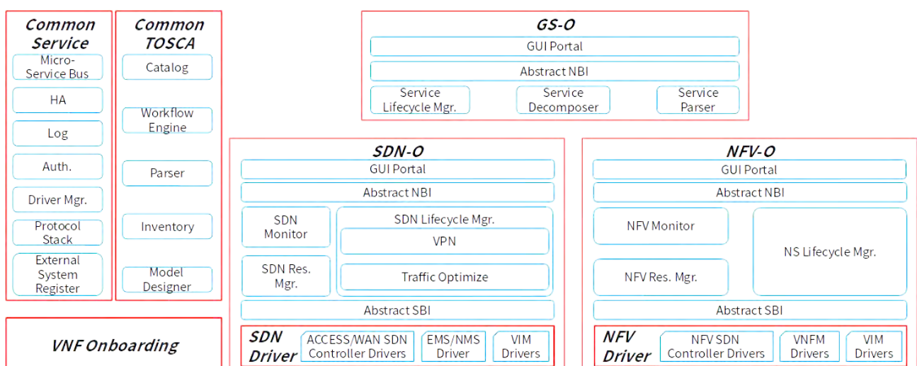
Figure 2.11: OPEN-O Architecture
