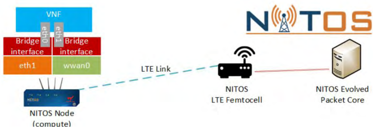
Figure 3.2: VNF deployment with LTE connectivity over the CITS NITOS LTE network
