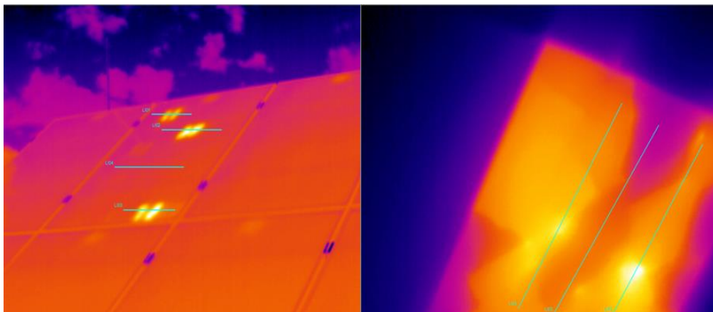
Figure 68 : Thermographic view taken from the front of the problematic PV panel with the cracked glass on the left. Close up view taken from the rear side of the same panel on the right where areas with different temperature are shown.
