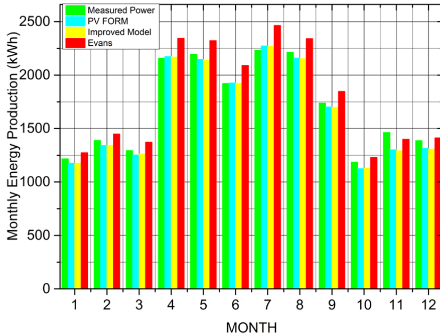
Figure 95 : Monthly Energy production (DC side) computed with the three models in comparison with the measured values for 2015
