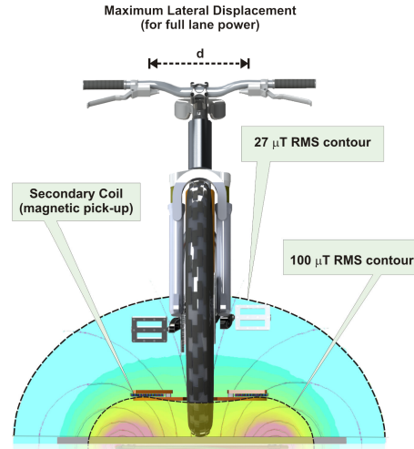
Figure 6. Front view of e-bike adapted with pick-up coil, represented on the inductive lane when its magnetic field is turned on.
