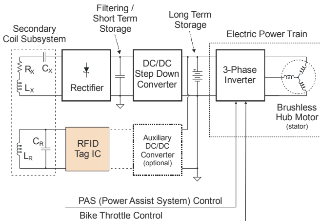
Figure 3. Diagram of the induction power receiver, on board of the e-bike.
