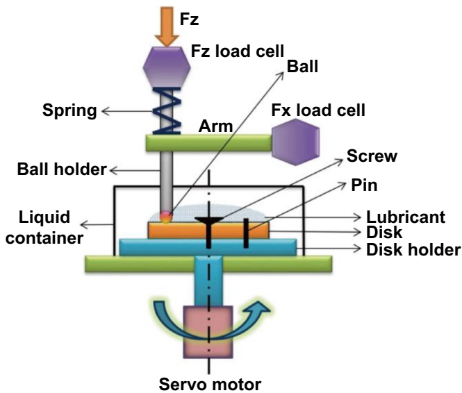
Figure 2. Schematic diagram of the ball-on-disk configuration used for tribological test.
