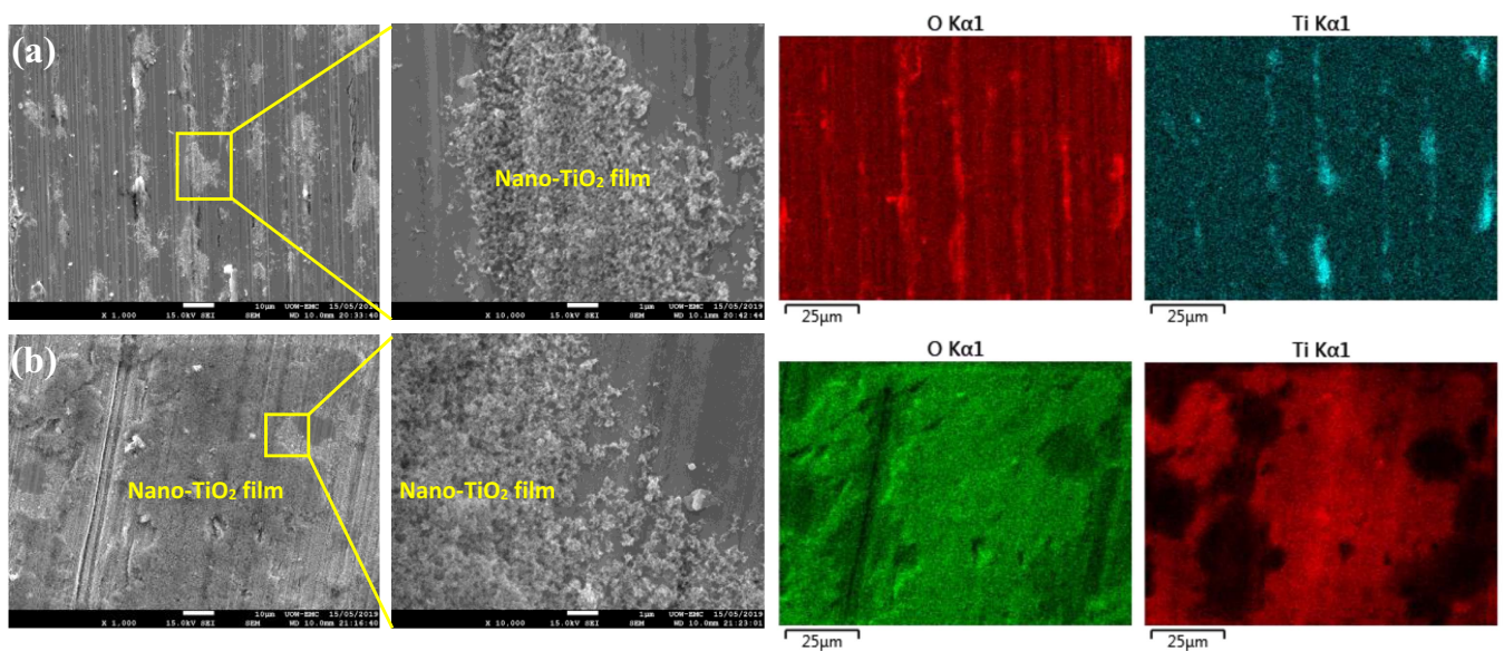
Figure 10. SEM images and EDS mappings of the wear tracks produced after tribological tests using (a) lubricant C and (b) lubricant D (30 N, 50 mm s -1 , 10 min).
