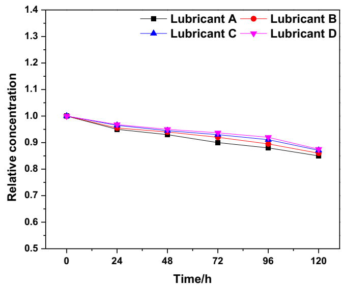
Figure 3. Dispersion stability of various water-based nanolubricants evaluated by using UV-vis spectrophotometer within 5 d.
