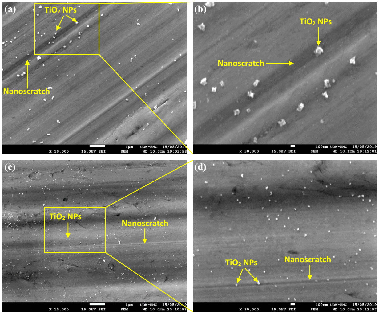
Figure 9. SEM images of the wear tracks produced after tribological tests using (a), (b) lubricant A and (c), (d) lubricant B (30 N, 50 mm s -1 , 10 min).
