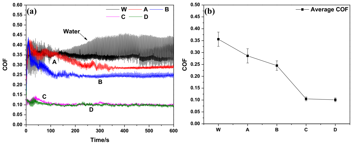
Figure 4. (a) COF curves over sliding time, and (b) averaged COF values obtained from the stable stages of sliding against Q345 disk under different lubrication conditions (30 N, 50 mm s -1 , 10 min).
