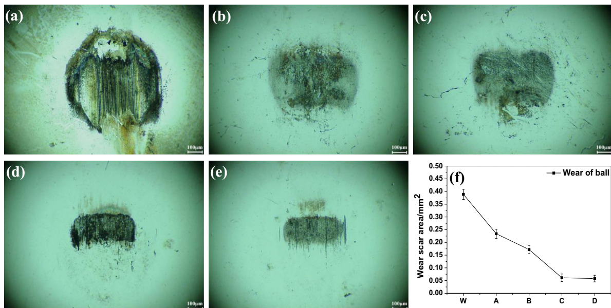
Figure 5. Surface morphologies of the worn balls obtained under (a) water, (b) lubricant A, (c) lubricant B, (d) lubricant C, (e) lubricant D, and (f) comparison of averaged wear scar areas (30 N, 50 mm s -1 , 10 min).
