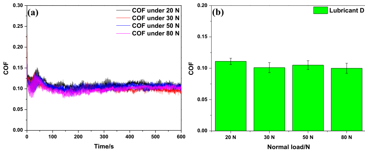
Figure 6. (a) COF curves over sliding time, and (b) averaged COF values obtained from the stable stages of sliding against Q345 disk under different loads ( 50 \text{ mm s}^{-1} , 10 min).
