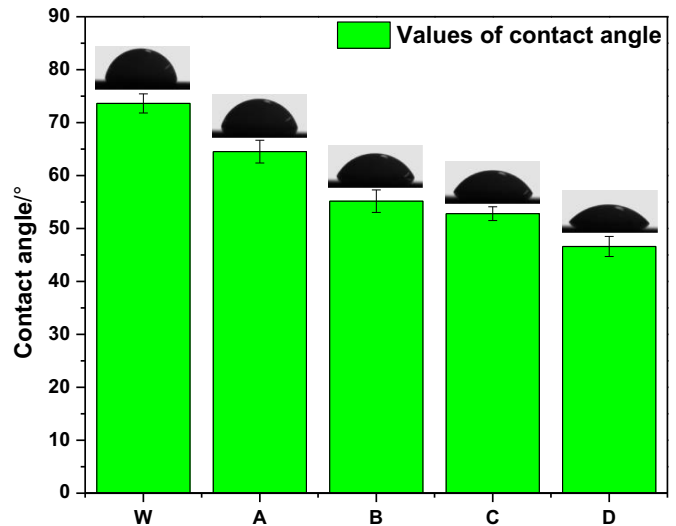
Figure 8. Contact angle values measured on HSS surface using different lubricants.
