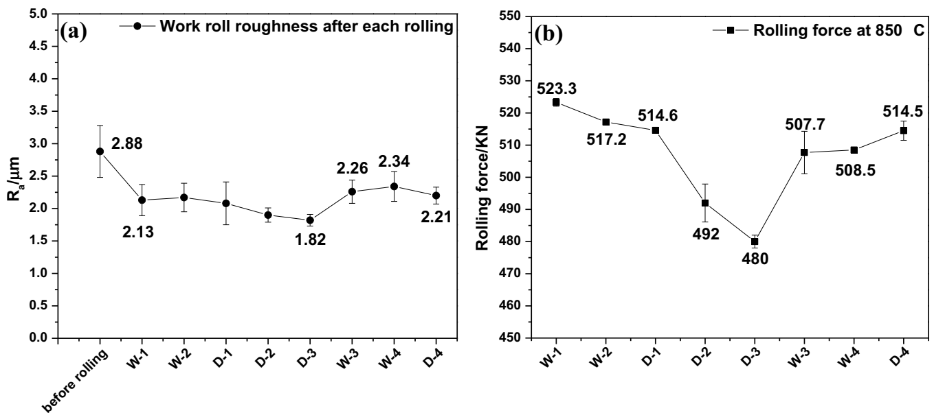
Figure 7. Variations of (a) work roll roughness and (b) corresponding rolling force under water and lubricant D at 850 \text{ }^\circ\text{C} .
