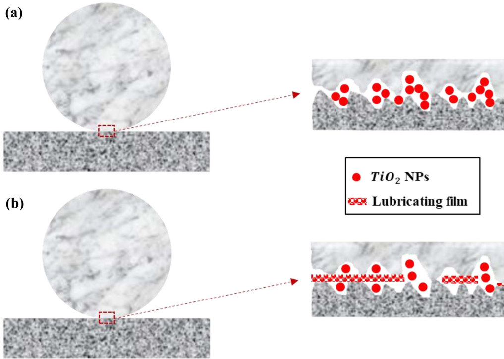
Figure 11. Schematic illustration of the lubrication mechanisms using (a) lubricants A and B, and (b) lubricants C and D.
