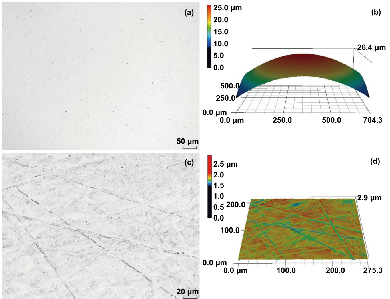
Figure 1. Surface morphologies and 3D profiles of (a), (b) E52100 Cr steel ball, and (c), (d) Q345 disk.
