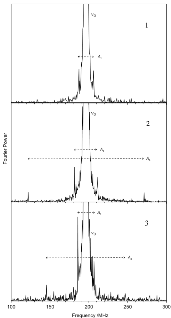
Figure 2. Transverse-field \mu SR spectra at 14.48 kG obtained from a solution of 1 in tetrahydrofuran at 53.5°C (upper), 2 in tetrahydrofuran at 53.7°C (middle), and 3 in tetrahydrofuran at 54.6°C (lower).
