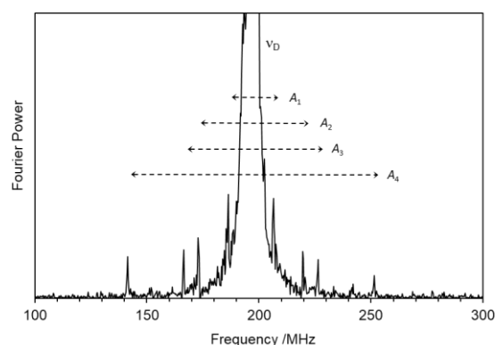
Figure 1. Transverse-field \mu SR spectrum at 14.48 kG obtained from a solution of 4 in hexane at 50.6°C. This Fourier transform corresponds to a 3 \mu s time window delayed by 85 ns. The truncated signal labelled V_D is due to muons in diamagnetic molecules, whose spins precess at the muon Larmor frequency (196.15 MHz at this magnetic field). A_1 , A_2 , A_3 and A_4 denote the separation of the pairs of radical precession frequencies and thus comprise the muon hyperfine constants.
