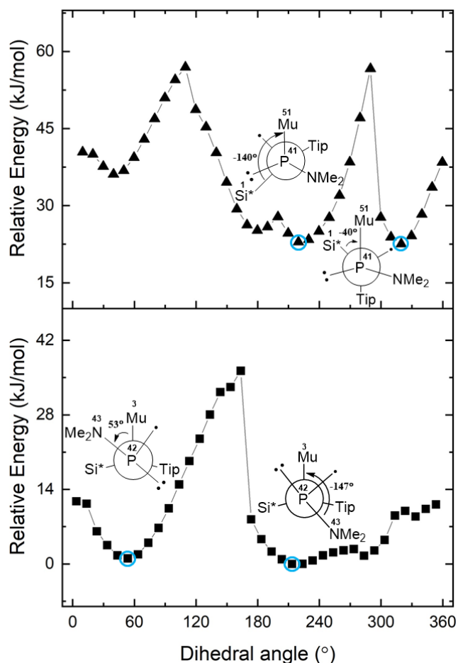
Figure 3. Potential energy surface scans for rotation about the Si-P bonds of radicals formed by Mu addition to phosphasilene 4 at the Si atom (lower) or the P atom (upper). The blue circles denote radical conformations detected by muon spin spectroscopy.
