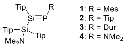
Scheme 1. Phosphasilenes investigated (CCDC No. for 2 : 1989736 and 3 : 1989735). Mes = 2,4,6-trimethylphenyl, Tip = 2,4,6-triisopropylphenyl, Dur = 2,3,5,6-tetramethylphenyl, NMe 2 = dimethylamino.
