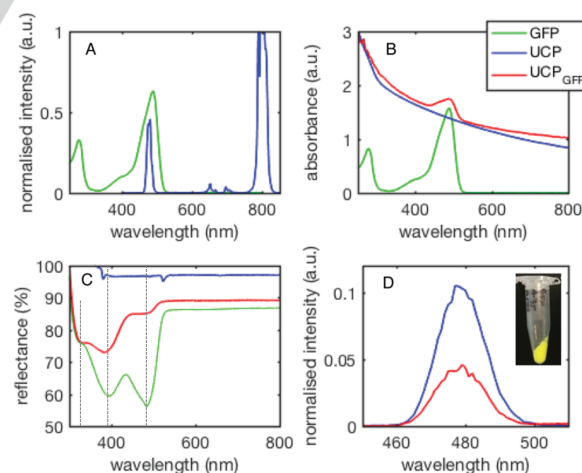
Figure 1. (A) Spectral overlap of GFP absorption (green) with UCP emission (blue). (B) Solution UV-vis absorption spectra of GFP, UCP, and UCP GFP in PBS. (C) Solid-state UV-vis reflectance spectra of GFP, UCP, and UCP GFP separately drop-cast and dried between two glass slides, with UCP GFP displaying distinct GFP bands. (D) Upconversion emission spectra of UCP and UCP GFP ( \lambda_{\text{ex}} = 980 nm) in PBS. Bands are normalized to the 800 nm UC emission intensity with full spectra shown in Figure S-3. (Inset) Photograph of UCP GFP showing distinct luminous yellow-green coloration from conjugated GFP. Universal legend for all panels: green = GFP, blue = UCP (PTIR-475), red = UCP GFP .
