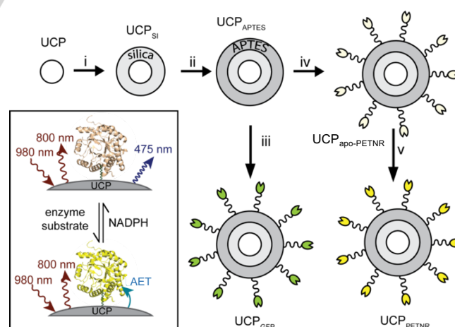
Scheme 1. Simplified representation of overall synthetic scheme; i) Igepal CO-520, NH 4 OH, TEOS, cyclohexane; ii) APTES, cyclohexane; iii) Sulfo-SMCC, GFP, PBS; iv) Sulfo-SMCC, PETNR, PBS; v) KBr, FMN, PBS; see SI for additional experimental details. Inset shows “on-off” apparent energy transfer (AET) concept with PETNR on the surface of UCPs.
