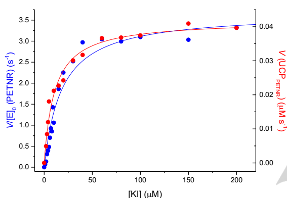
Figure 3. Michaelis-Menten plots for the reaction of PETNR (blue) and 1 \text{ mg ml}^{-1} UCP PETNR (red) with 100 \mu\text{M} NADPH and varying substrate, KI. These data are fitted to Eq. 1 (solid lines).
