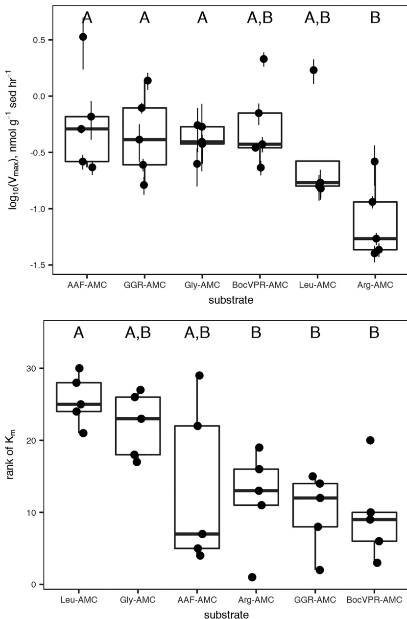
FIG 2 V_{max} and K_m values, shown individually with error bars indicating SEs of the nonlinear least-squares estimates, and collectively in a box-and-whisker plot. Substrates sharing a letter are not significantly different according to one-way analysis of variance (ANOVA) of \log_{10} -transformed data with Tukey honestly significant difference (HSD) post hoc analysis ( V_{max} ) or Kruskal-Wallis test with Tukey HSD post hoc analysis ( K_m ).
