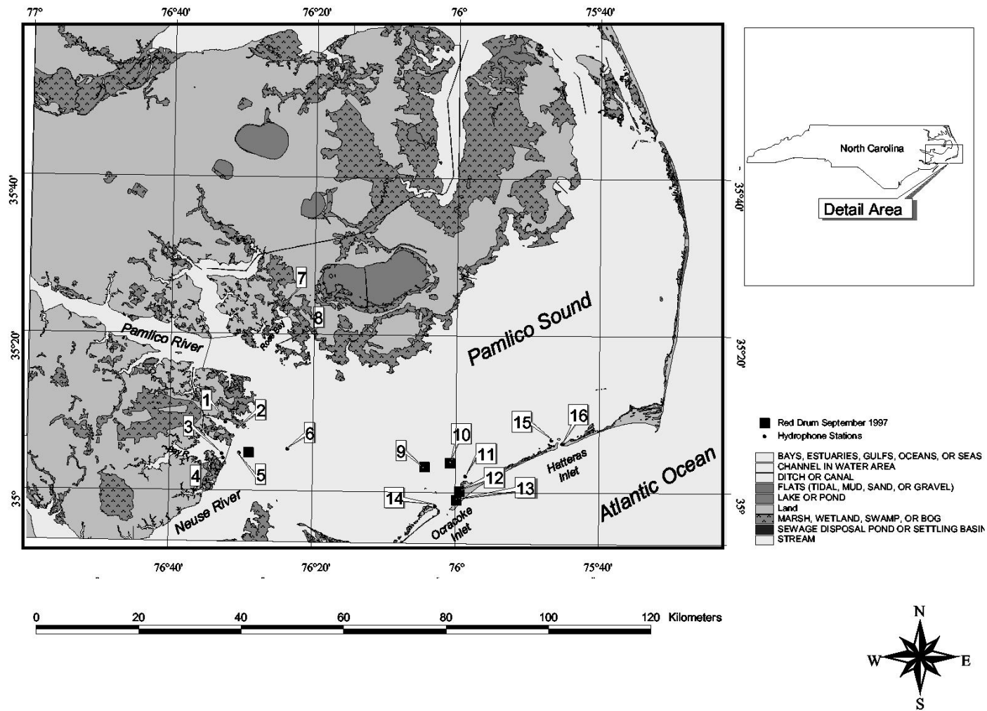
Figure 28. Locations in which red drum were heard making "knocking" sounds in September 1997.
