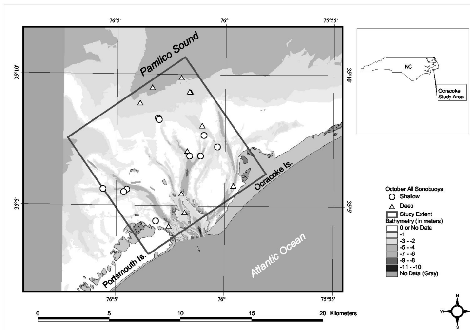
Figure 9. Random positions of all sonobuoys in October 1998 at Ocracoke. Symbols indicate deep and shallow locations
