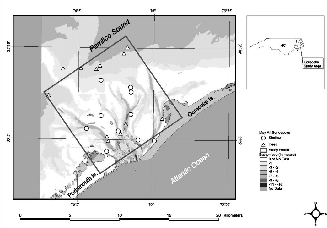
Figure 4. Random positions of all sonobuoy in May 1998 at Ocracoke. Symbols indicate deep and shallow locations.
