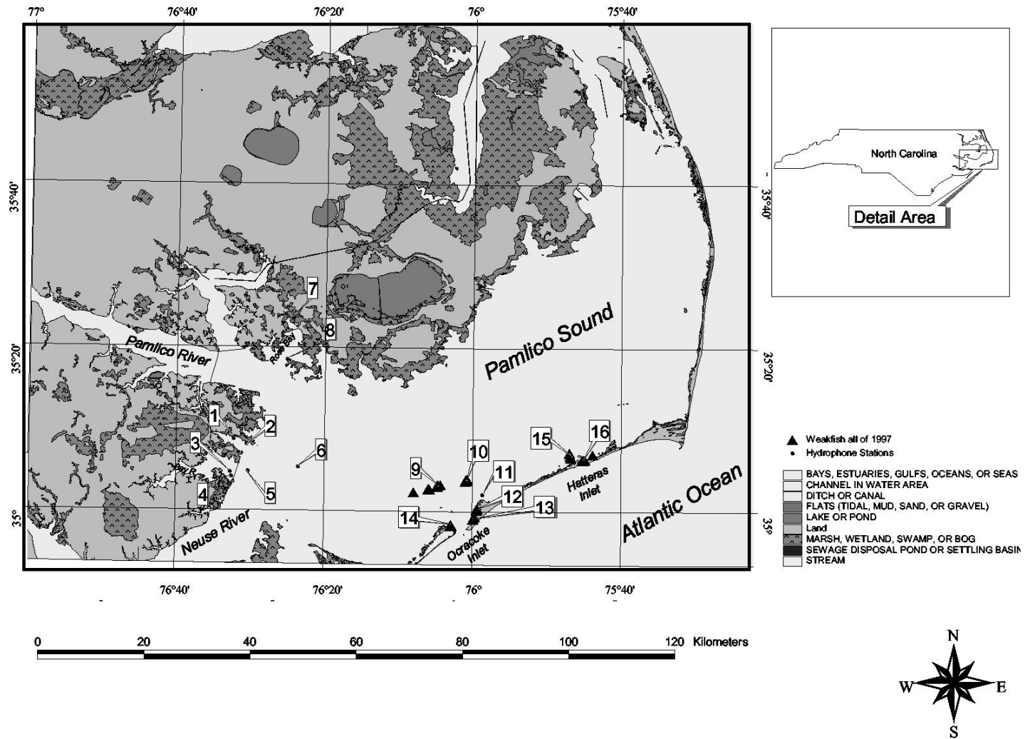
Figure 20. A map showing the locations where weakfish "purring" was recorded during the hydrophone survey in 1997.
