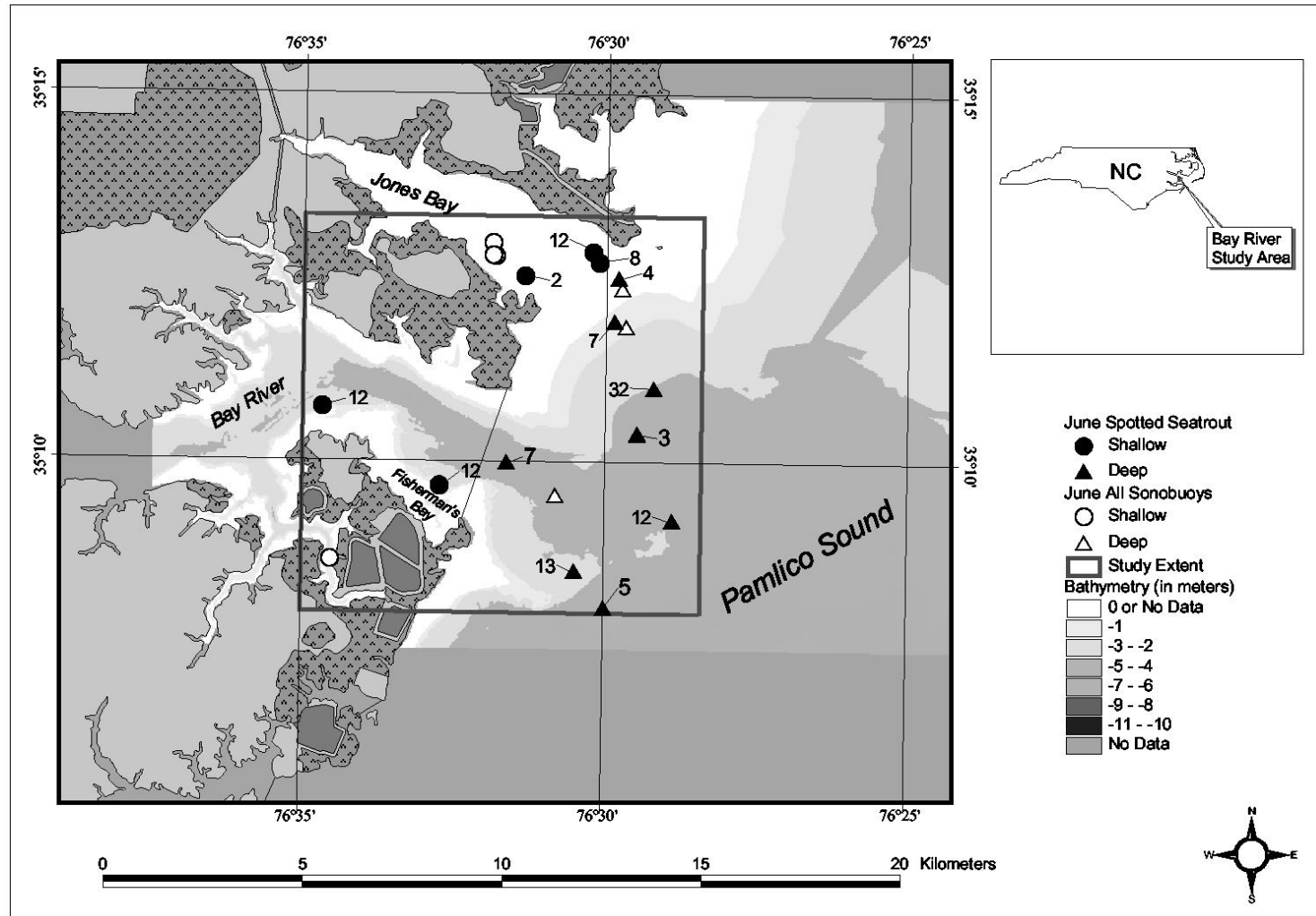
Figure 66. A map of the Bay River study area showing shallow ( < 10' ) and deep ( > 10' ) sonobuoy locations in June 1998. Filled symbols represent stations in which spotted seatrout "heartbeat," "burp" or "staccato" sounds were detected on a sonobuoy tape. The number next to each symbol represents the drumming index sum for the sonobuoy recording at that location (see text).
