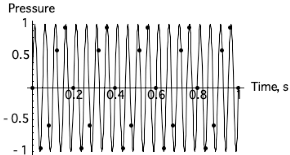
Figure 75. Discrete sampling of a signal. The dots are the sample points.
