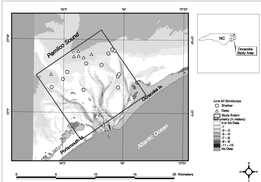
Figure 5. Random positions of all sonobuoy in June 1998 at Ocracoke. Symbols indicate deep and shallow locations.
