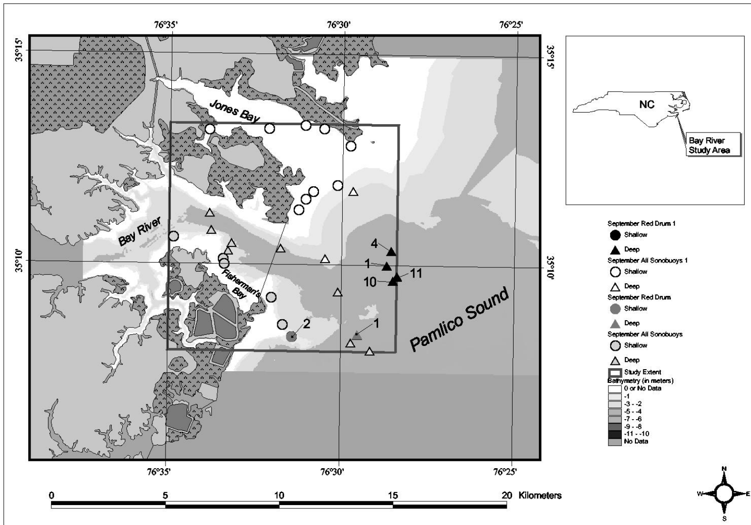
Figure 74. A map of the Bay River study area showing shallow ( < 10' ) and deep ( > 10' ) sonobuoy locations in September 1998. Filled symbols represent stations at which red drum "knocking" sounds were detected on a sonobuoy tape. The number next to each symbol represents the drumming index sum for the sonobuoy recording at that location (see text).
