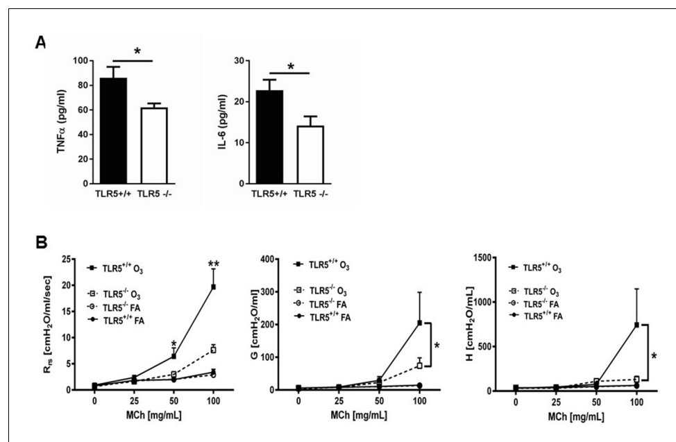
Figure 2. TLR5 deficiency ameliorates the in vivo inflammatory response to inhaled O 3 . (A) TNF- \alpha and IL-6 levels in the lung lavage fluid of Tlr5 -deficient ( Tlr5 -/- ) or Tlr5 -competent ( Tlr5 +/+ ) mice 24 hr after receiving 3 ppm O 3 for 3 hr by inhalation. n = 14 mice for Tlr5 +/+ and n = 12 mice for Tlr5 -/- , experiment repeated twice. (B) Airway physiology measurement (total respiratory resistance R rs , tissue damping G and tissue elastance H) to indicated doses of methacholine challenge measured with flexiVent in Tlr5 -deficient ( Tlr5 -/- ) or Tlr5 -competent ( Tlr5 +/+ ) mice 24 hr after 2ppm O 3 or air (FA) exposure. n = 6 for Tlr5 -/- FA and Tlr5 -/- O 3 and n = 7 for Tlr5 +/+ FA and Tlr5 +/+ O 3 , experiment repeated three times. Data are represented as mean \pm s.e.m. and were analyzed by unpaired t test with Welch's correction *p<0.05 and **p<0.01 between Tlr5 +/+ and Tlr5 -/- mice exposed to O 3 .
