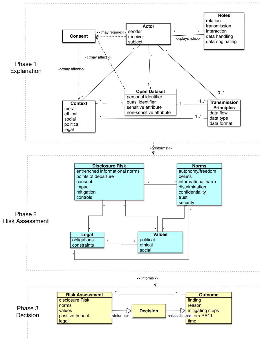
Figure 3. Meta-model of contextual integrity.
