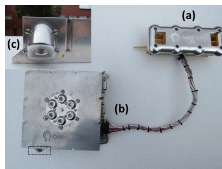
Figure 1: Image of the HABIT instrument. (a) Container Unit (CU), (b) Electronic Unit (EU) with Ground Temperature Sensor (GTS) highlighted, (c) a closer view of the GTS pointing at the surface.
