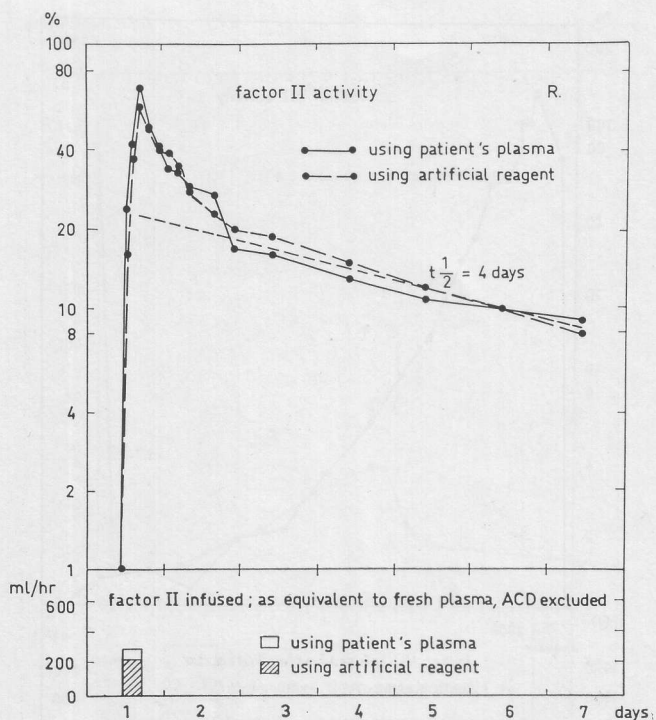
Fig. 4. Results of infusion of Prothrombin; patient GK 314/68; 26-year-old male; Factor II approximately 1% of normal; plasma volume 3 liters.
