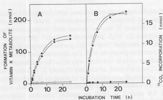
FIG. 2. Time course of the formation of vitamin K epoxide (●—●), hydroxyvitamin K (○—○), and the ^{14}\text{CO}_2 incorporation (■—■). All data are expressed as nmol/mg of carboxylase. A, in the absence of sulfite; B, in the presence of 60 mM disodium sulfite.
