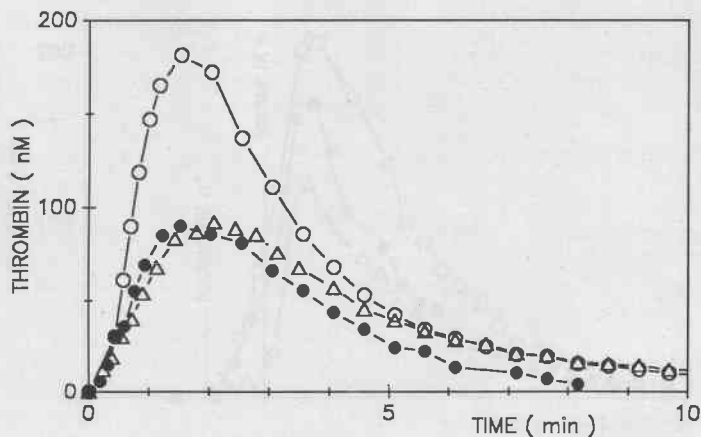
Fig. 3 Thrombin generation in plasma after triggering with complete tenase. Trigger: factor IXa (1.2 nM), factor VIIIa (1.6 U/ml), phospholipid (1.2 \mu\text{M} ) (final concentrations) and \text{Ca}^{2+} (see methods). Symbols as in Fig. 1
