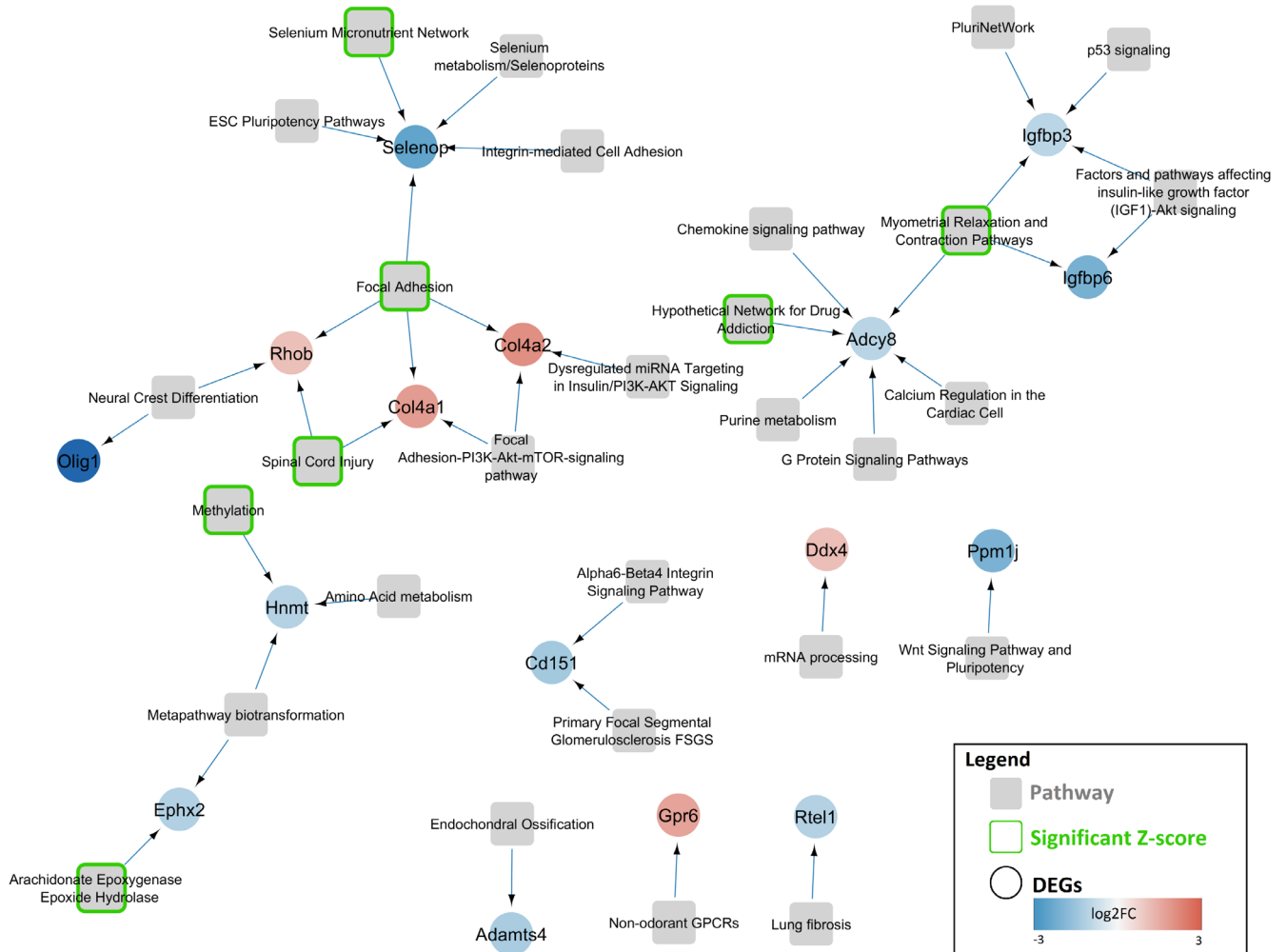
Figure 2. Gene-Pathway network for differentially expressed genes (DEGs) in Purkinje cells of Mecp2 -y vs. wild type. DEGs in a mouse model for Rett syndrome ( Mecp2 -y mice) were selected and imported in Cytoscape (circular nodes). The genes are colored based on changes in gene expression (blue=down-regulated, red=up-regulated). Thereafter, gene-pathway associations from WikiPathways were added and the pathways are shown as gray rectangles. Genes without pathway annotations have been removed. The green border color indicates pathways that are significantly altered based on over-representation analysis in PathVisio (Z-Score > 1.96).
