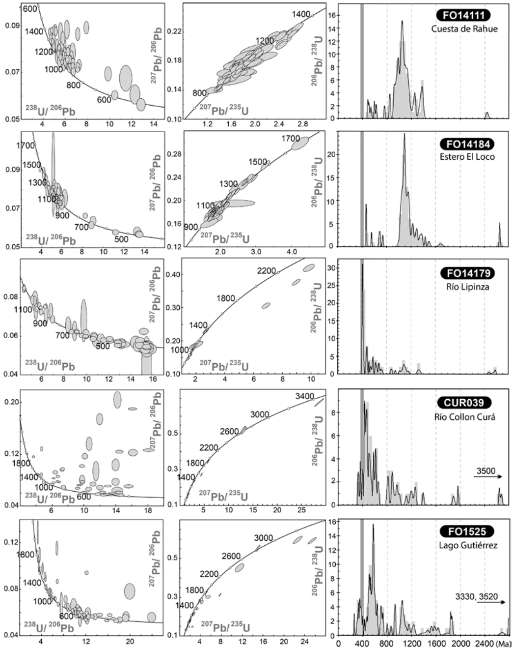
FIG. 3. Tera-Wasserburg (data uncorrected for common Pb), Wetherill ( ^{204}\text{Pb} -corrected) and preferred age versus frequency/relative probability diagrams for metasedimentary rock sample zircon from the eastern (continental) Devonian belt (continued in figure 4)
