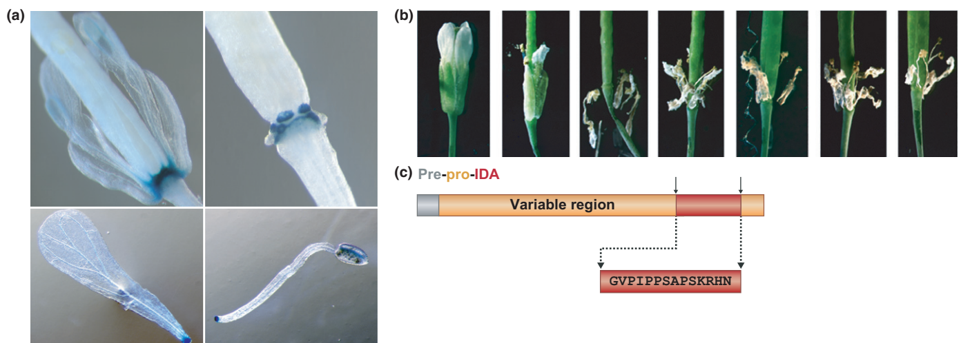
Fig. 5 Subtilases (SBTs) in Inflorescence Deficient in Abscission (IDA) maturation and floral organ abscission. (a) Promoter:reporter ( uidA ) gene analysis indicates expression of SBTs in the abscission zones of floral organs in Arabidopsis flowers. (b) Floral organs do not abscise when SBT activity is inhibited in abscission zones by tissue-specific expression of the SBT-specific EPI10 inhibitor (Schardon et al. , 2016). (c) Precursor processing by several functionally redundant SBTs is required for the biogenesis of the mature IDA peptide (GVPIPPSAPSKRHN; Schardon et al. , 2016).
