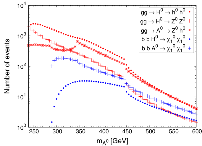
Fig. 6. Number of events expected at the LHC for H^0 \rightarrow h^0 h^0 , Z^0 Z^0 and A^0 \rightarrow Z^0 h^0 through Higgs production via gluon fusion (in red), and (H^0, A^0) \rightarrow \tilde{\chi}_1^0 \tilde{\chi}_1^0 through Higgs production associated with a pair of bottom quarks (in blue), for a total integrated luminosity of \mathcal{L} = 23 \text{ fb}^{-1} and a center-of-mass energy of \sqrt{s} = 8 \text{ TeV} . The input parameters are chosen as in Fig. 5: M_S = 35 \text{ TeV} , m_S = 7.5 \text{ TeV} , A_t = 0 , M_1 = 150 \text{ GeV} , M_2 = 1 \text{ TeV} , M_3 = 3 \text{ TeV} , \mu = 300 \text{ GeV} and \tan\beta = 7.5 . (For interpretation of the references to color in this figure legend, the reader is referred to the web version of this Letter.)
