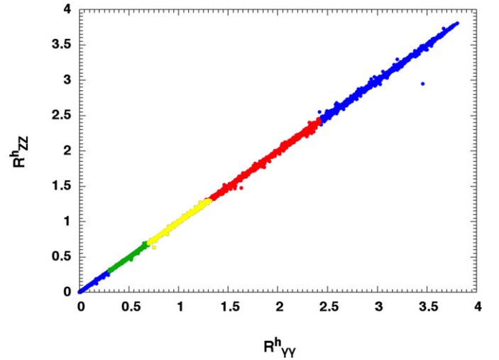
Fig. 3. Correlation between \gamma\gamma and ZZ signal rates for the light Higgs boson h^0 . Red and green dots are for 0.7 < R_{\gamma\gamma}^h < 2.42 (95% C.L.) and 0.3 < R_{ZZ}^H < 1.3 (95% C.L.), respectively; yellow dots represent points of the parameter space that fulfill both previous requirements; blue dots do not satisfy any of them. (For interpretation of the references to color, the reader is referred to the web version of this Letter.)
