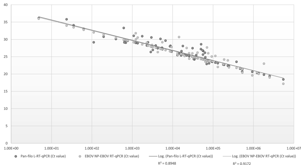
Fig. 2. Parallel results of pan-filo L-RT-qPCR (this study) and EBOV NP-RT-qPCR [20] assays. The RNA copy numbers (5 copies to 5.5 million copies) of EVD patient samples are presented in the X-axis (logarithmic scale, \log_{10} ) and Ct values in the Y-axis. R^2 , R-squared.
