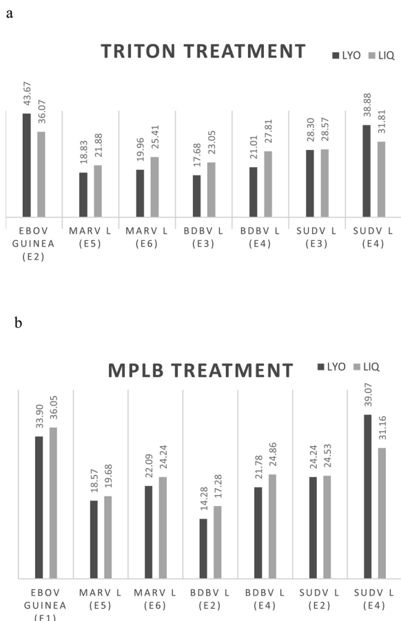
Fig. 1. (a) and (b) Comparing the performance of the pan-filo L-RT-qPCR using Thermo-lyophilized and Invitrogen-liquid assays for potential inhibitory effects of different reagents and inactivation methods [Fig. 1a., Triton™-X 100 treatment (Triton) or Fig. 1b. Magna Pure Lysis buffer (MPLB)].
