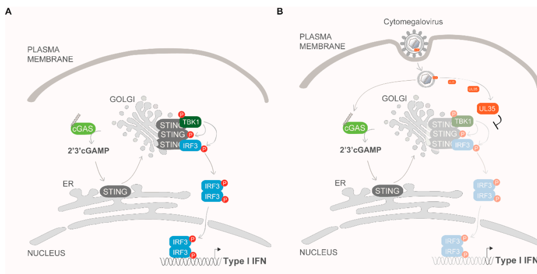
Figure 8. UL35 targets TBK1 to antagonize type I IFN signaling. Nucleic acids (A) or CMV infection (B) are recognized via sensors such as cGAS, which triggers signaling via TBK1 and IRF3 to induce transcription of IFN \beta . (B) Following viral entry, tegument UL35 targets TBK1 to downmodulate the type I IFN response.
