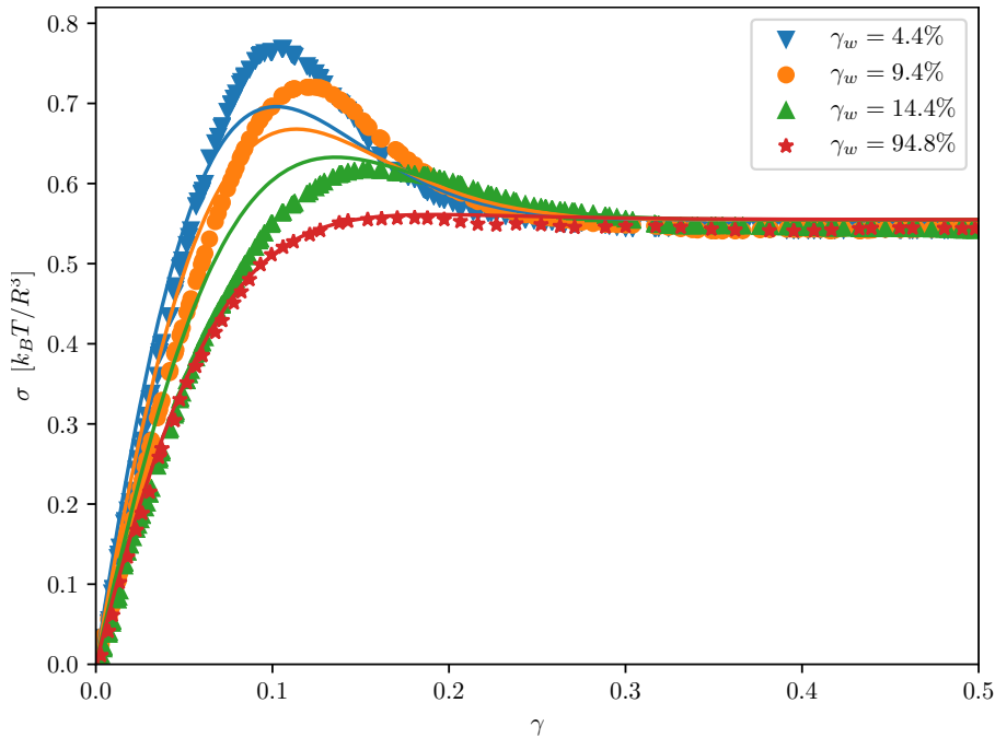
Fig. 6 Symbols: Stress–strain curves of a colloidal hard-sphere-like suspension (PS-PNiPAM particles, R \approx 90 nm) after different amounts of pre-strain \gamma_w in the opposite direction, at a shear rate of \dot{\gamma} = 5 \times 10^{-4} \text{ s}^{-1} . Lines: Results from a generalized Maxwell model (see text).
