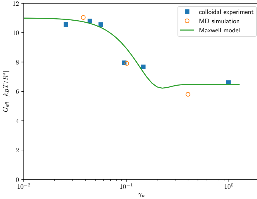
Fig. 7 Filled symbols: Effective shear modulus G_{\text{eff}} = \Delta\sigma/\Delta\gamma obtained from the colloidal stress–strain curves shown in Fig. 6. Open symbols: from MD simulations of a typical molecular glass former (data from Ref. [93]). Line: Prediction from a generalized Maxwell model (see text; scaled by 11/15 to match the experimental shear modulus at \gamma_w = 0 ).
