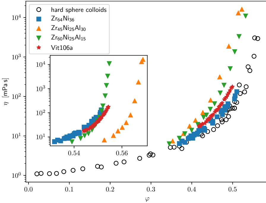
Fig. 1 Viscosity of selected metallic melts (filled symbols as labeled; Zr_{64}Ni_{36} from experiment [35]; Zr_{75-x}Ni_{25}Al_x from molecular dynamics simulations [36]; Vit106a, Zr_{58.5}Cu_{15.6}Ni_{12.8}Al_{10.3}Nb_{2.8} from experiment [37]) as a function of empirical packing fraction \phi , compared with the viscosity obtained from various hard-sphere like colloidal suspensions (collected in and taken from Ref. [38]; assuming a solvent viscosity of 1 mPas). Main panel: using empirical diameters d_{\text{eff},\alpha} = d_{\alpha}(T/T_0)^{-n} , with n = 0.2 and T_0 = 950 K and d_{\alpha} from Pauling [34]; inset: using d_{\alpha} without temperature correction.
