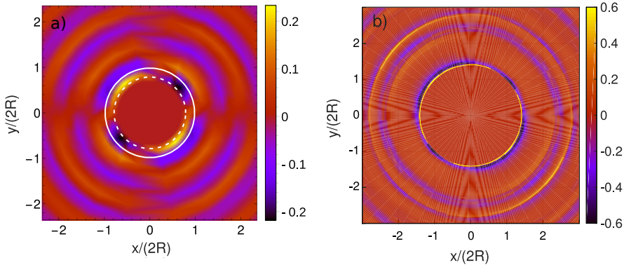
Fig. 3 Distortion of the radial distribution function, \delta g(\vec{r}) = g(\vec{r}; \dot{\gamma}) - g_{\text{eq}}(r) , under shear flow of rate \dot{\gamma} , displayed in the shear–shear-gradient plane ( x : direction of flow, y : direction of gradient). a) from molecular-dynamics (MD) simulations of a model of Ni; b) from Brownian dynamics (BD) simulations of a binary hard-sphere system with size ratio \delta = 0.8 . Dashed and solid white circles are guides to the eye to emphasize cuts of constant r where l = 2 and l = 4 deformations can be seen (two minima interspersed by two maxima, respectively four separated minima).
