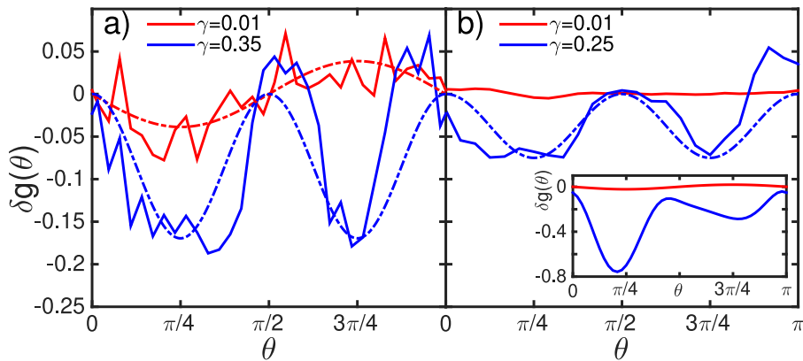
Fig. 5 Angular dependence of g(\vec{r}) at fixed radial distance r \approx 2R , as a function of the angle to the shear-flow direction, \theta , for two strains \gamma after startup flow before ( \gamma = 0.01 : top curves) and after ( \gamma > 0.1 : bottom curves) the yield strain. Dash-dotted lines are fits using a quadrupole signal \sin 2\theta (top) and a hexadecupolar signal (\sin 2\theta)^2 (bottom). a) From MD simulation of liquid Ni. b) From confocal microscopy of a PMMA hard-sphere colloidal suspension ( r = 2.1R ). Inset: Results from mode-coupling theory (ITT-MCT) for a 2D hard-disk system.
