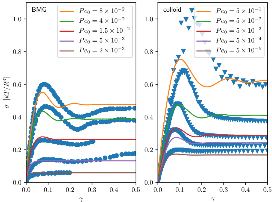
Fig. 2 Stress \sigma versus strain \gamma for different deformation rates given as Péclet numbers Pe_0 . Left: for a bulk metallic glass (Vitreyloy 1, Zr_{41.2}Be_{22.5}Ti_{13.8}Cu_{12.5}Ni_{10} , T = 613 K, from Ref. [59]; strain rate rescaled by \sqrt{3} to account for the deformation geometry, see text). Right: for colloidal hard spheres (PS-PNiPAM, \phi \approx 0.60 , from Ref. [60]). Lines are fits using a sheared-hard-sphere model of MCT in isotropic approximation (see text for details), rescaled by 0.75 and 0.32 for the BMG and the colloidal sample, respectively, and using strain-scale parameters of \gamma_c = 0.3 and \gamma'_c = 0.12 (BMG; left), and \gamma_c = 0.3, 0.2, 0.2, 0.1 and \gamma'_c = 0.18, 0.16, 0.14, 0.14, 0.14 (colloid for increasing Pe_0 ; right), see Appendix A for details.
